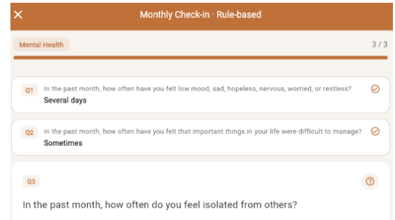
Fig. 4. Rule-based monthly check-in for Sophie’s Month 2 Mental Health scenario. The branching engine presents three generic questions; the functional-impact item is hidden because the mood-frequency threshold is not met.
