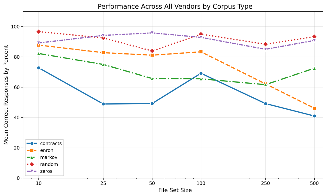
Figure 4: Performance by Corpora
