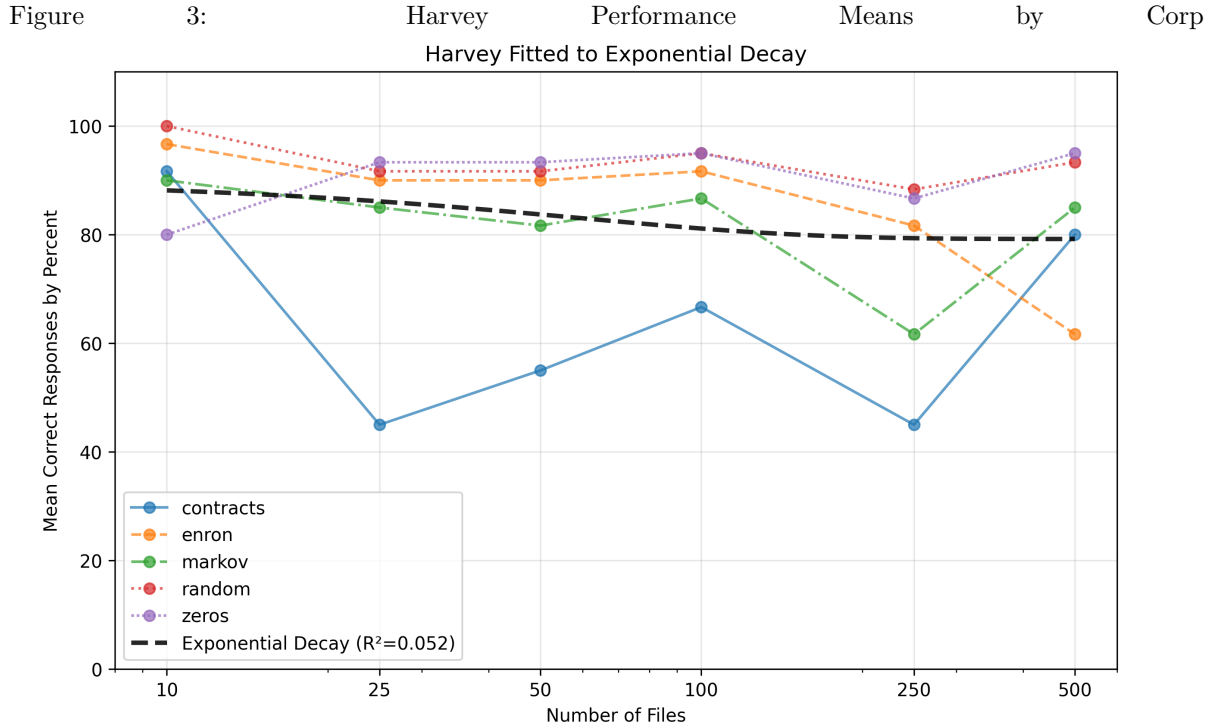
Caption: A line graph showing the performance of the Harvey platform on retrieval performance. Each line represents a different corpus. A separate line showing a fitted exponential decay function is overlaid, although its poor fit is noted.
