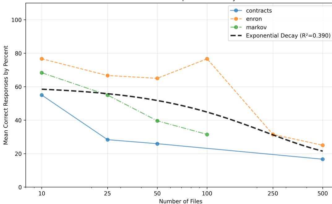
Figure 1: Lexis Performance Means by Corp Lexis Fitted to Exponential Decay
