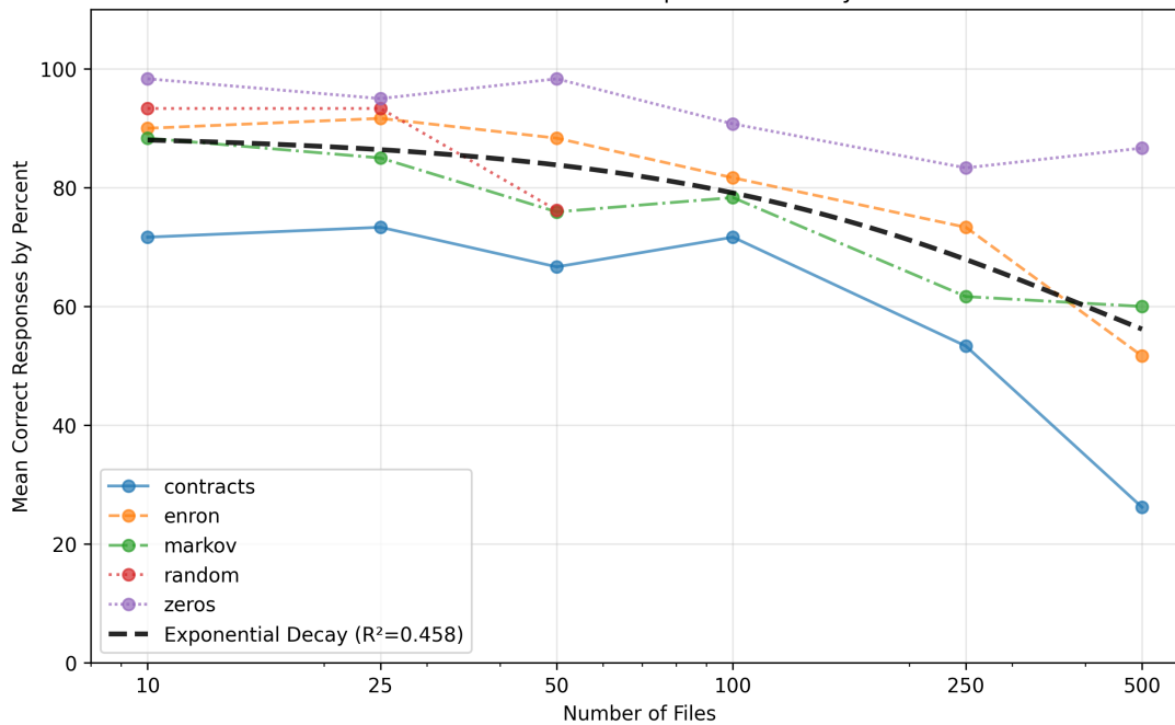
Figure 2: Westlaw Performance Means by Corp Westlaw Fitted to Exponential Decay
