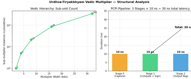
Fig. 6. Vedic multiplier hierarchy and PCPI pipeline analysis.
