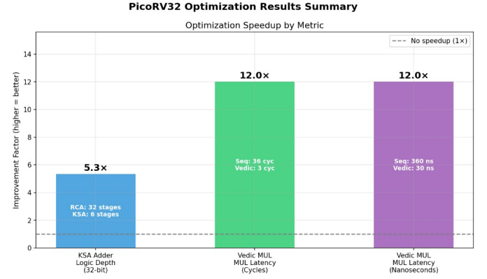
Fig. 7. Summary of measured optimization gains.
