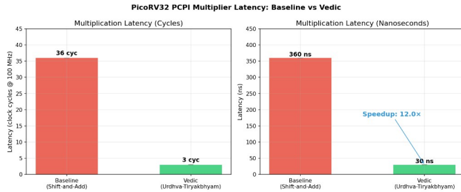
Fig. 2. PCPI multiplier latency comparison in cycles and nanoseconds.
