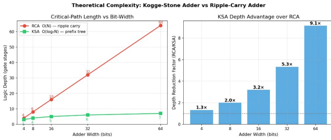
Fig. 5. Theoretical logic depth comparison for RCA versus KSA.
