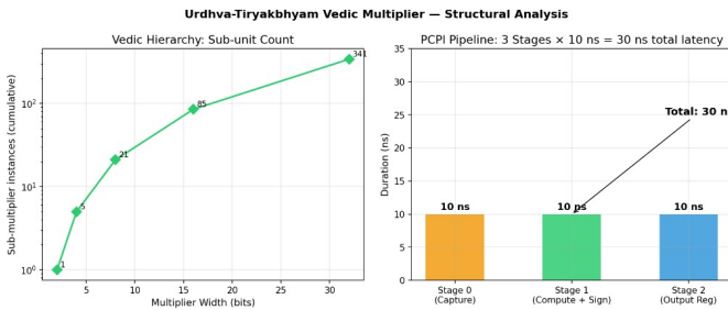
Fig. 6. Vedic multiplier hierarchy and PCPI pipeline analysis.
