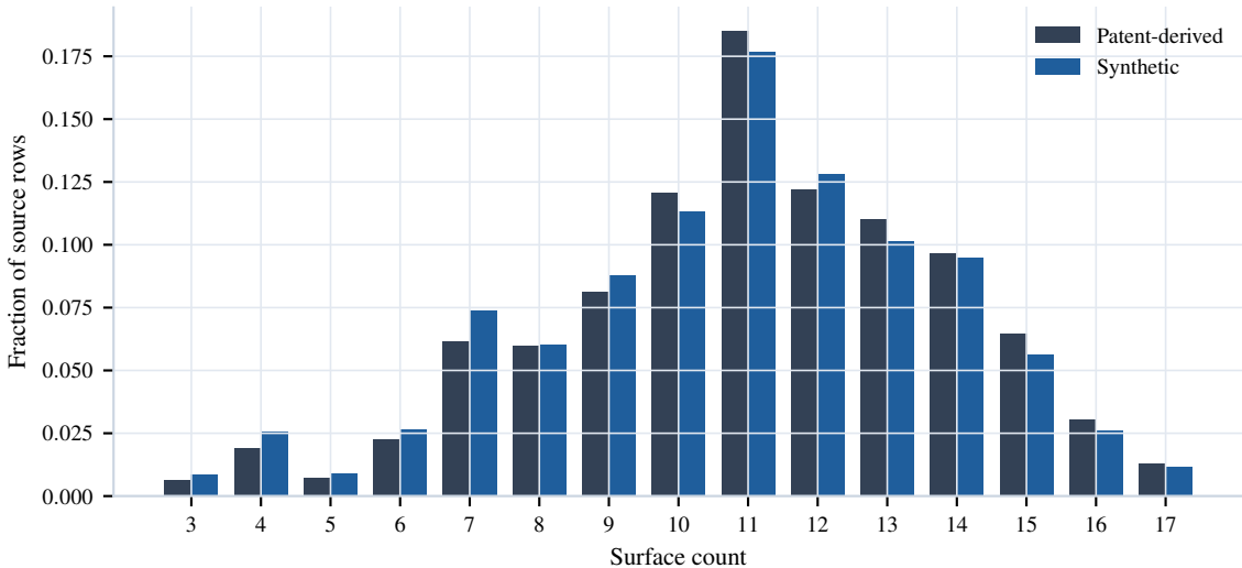
Surface-count coverage in patent-derived and synthetic rows
