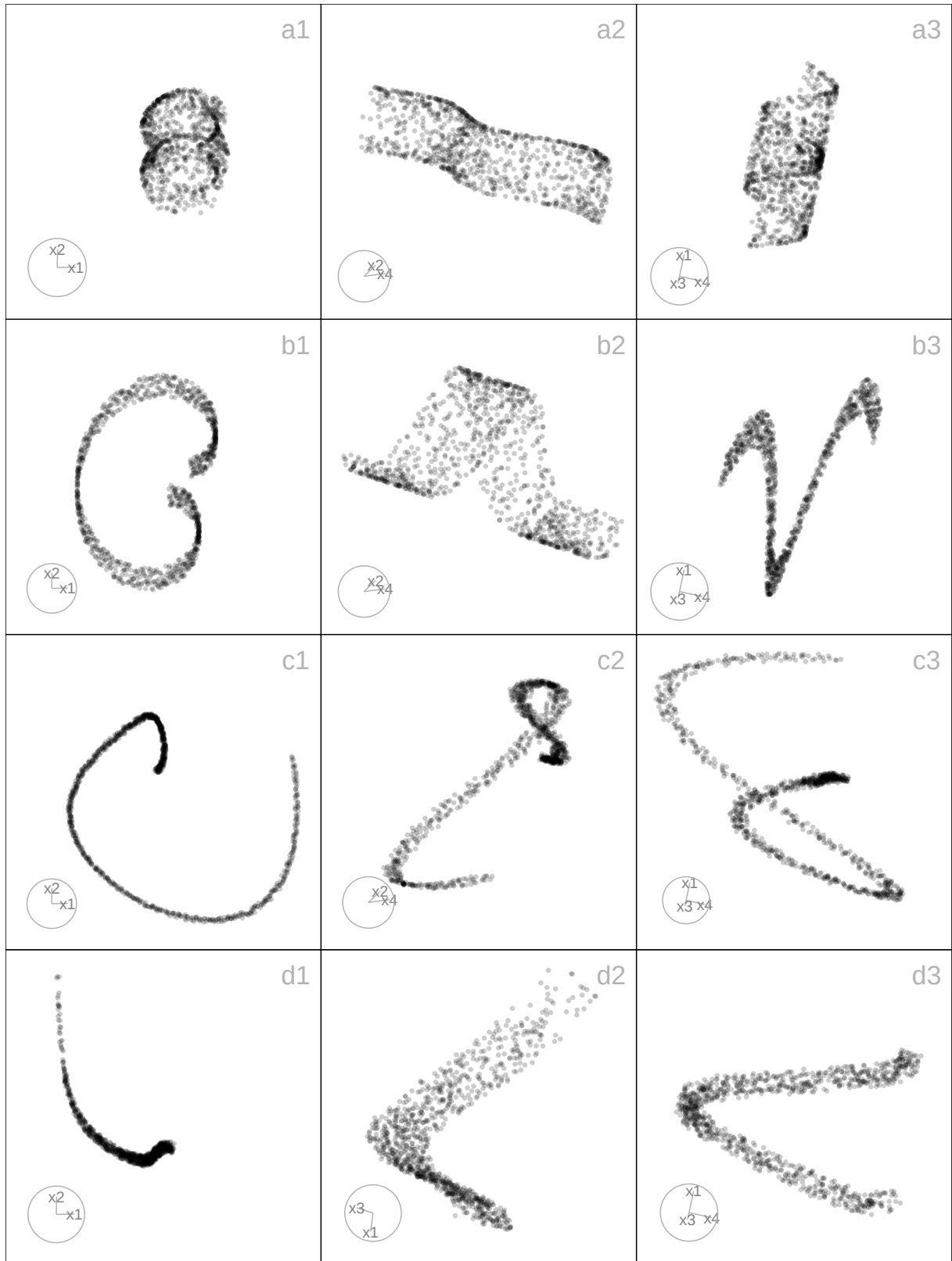
Figure 7.6: Three 2-D projections from 4-D, for the curvycylinder (a1-a3), sphericspiral (b1-b3), conicspiral (c1-c3), and nonlinear (d1-d3) data. The curvycylinder shows a cylindrical manifold with a nonlinear twist along its height, producing smooth, continuous curvature. The sphericspiral forms a spiral path on a spherical surface, combining circular and vertical motion in a helical form. The conicspiral spreads radially while ascending, forming a conical helix with twisting variations in a non-radial dimension. The nonlinear dataset exhibits a warped 2-D surface with sharp oscillations and smooth waves, reflecting complex nonlinear interactions. Each shows variations in curvature, density, and continuity.
