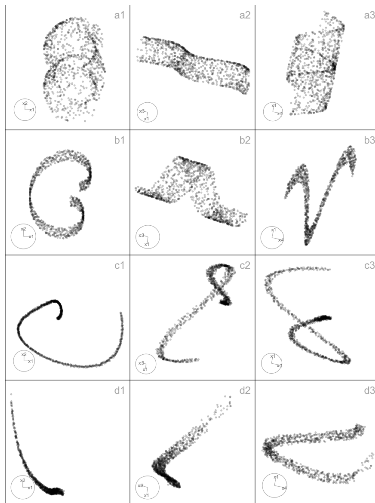
Figure 7: Three 2-D projections from 4-D, for the curvcylinder (a1-a3), sphericalspiral (b1-b3), conicspiral (c1-c3), and nonlinear (d1-d3) data. The curvcylinder shows a cylindrical manifold with a nonlinear twist along its height, producing smooth, continuous curvature. The sphericalspiral forms a spiral path on a spherical surface, combining circular and vertical motion in a helical form. The conicspiral spreads radially while ascending, forming a conical helix with twisting variations in a non-radial dimension. The nonlinear dataset exhibits a warped 2-D surface with sharp oscillations and smooth waves, reflecting complex nonlinear interactions. Each shows variations in curvature, density, and continuity.
