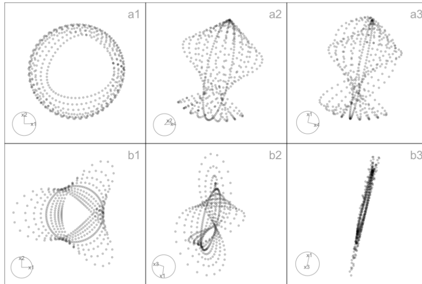
Figure 6: Three 2- D projections from 4- D , trefoil4d (a1-a3) and 3- D trefoil3d (b1-b3) data. The trefoil4d structure represents a higher-dimensional extension of the classic trefoil knot, revealing complex twisting and looping patterns that remain continuous across projections. In contrast, the trefoil3d dataset maintains a simpler, more compact knot-like form, showing how dimensional extension adds curvature and separation in the embedded space. These projections illustrate a range of looping structures in high-dimensions.
