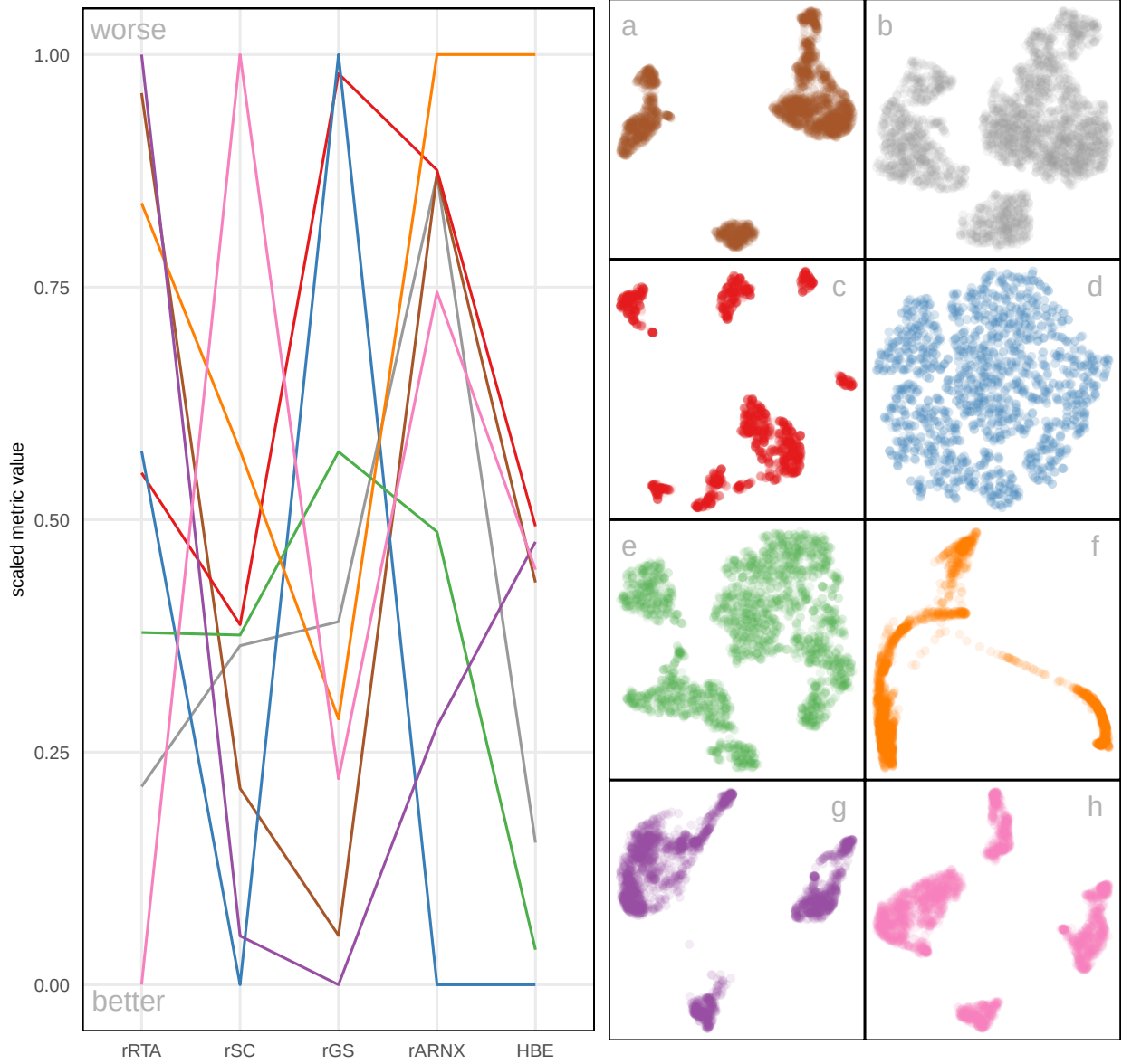
Figure 10: Comparison of scaled evaluation metrics (rRTA, rSC, rGS, rARNX, and HBE with a_1 = 0.06 ) for the eight NLDR layouts computed on the PBMC3k data, shown as a parallel coordinate plot. The color of each line corresponds to a NLDR layout. All, except rGS and rARNX agree that layout e is best or very close to best. Layout d is best according to HBE and rARNX but considered to be much less optimal by rRTA, rSC and rGS. Layout f is considered poor by rARNX and HBE. Layout a is considered close to the best by rGS and rSC.
