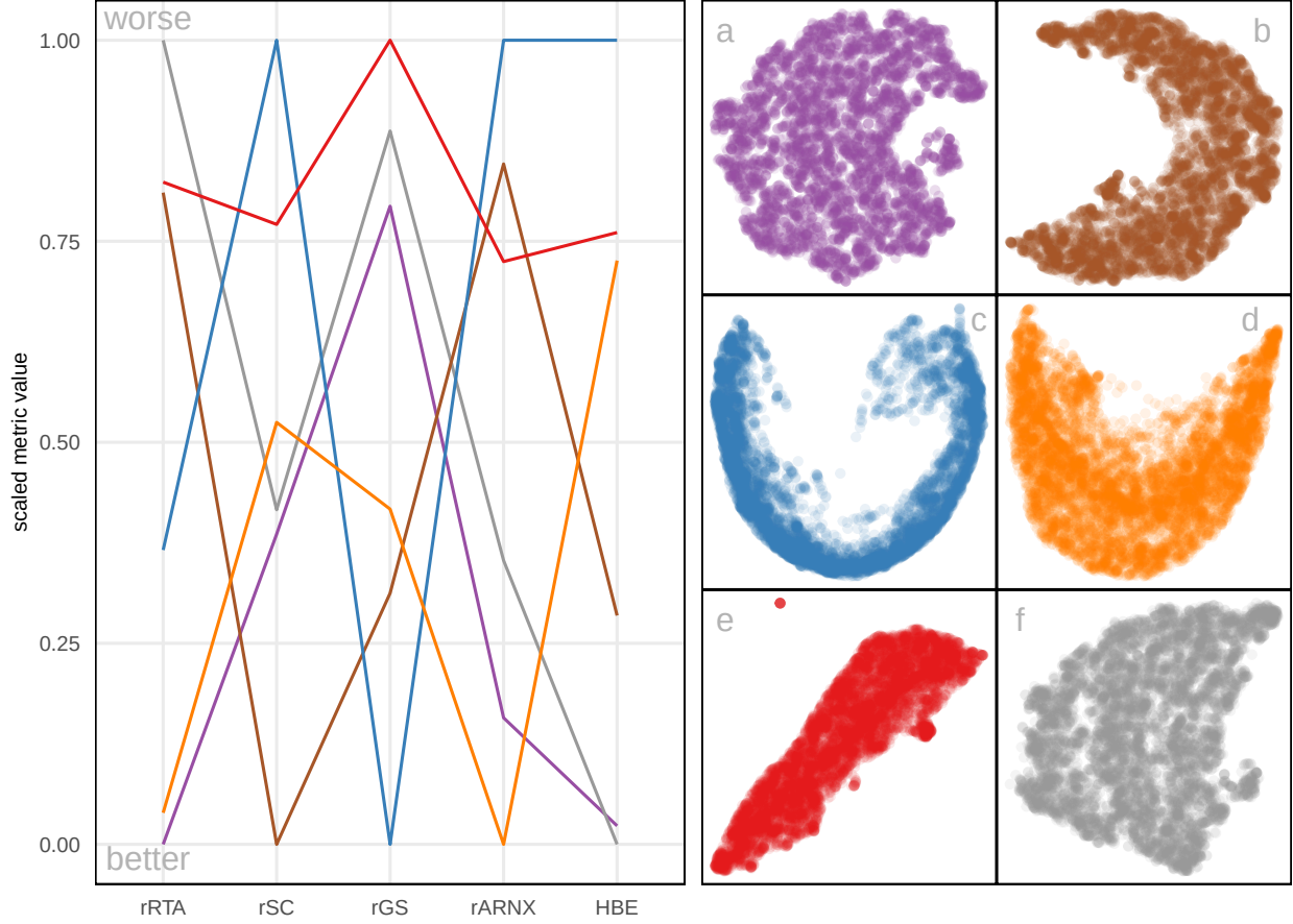
Figure 11: Comparison of scaled evaluation metrics (rARNX, rRTA, rSC, rGS, and HBE using a_1 = 0.04 ) for six NLDR layouts computed on the MNIST digit 1 data using a parallel coordinate plot. Each line represents a layout (a–f), with colors corresponding to the scatterplots shown on the right. The metrics display different ranking patterns, indicating that no single measure fully captures embedding quality. Layout a is identified as the best according to HBE and rRTA, but is considered much less optimal by rARNX, rSC, and rGS. Layout e is considered the worst, or close to the poorest, by all metrics. Layouts a and f show similar patterns of agreement across metrics, except for rRTA, where layout a performs the best and layout f the worst. Layout c is the worst in rARNX, rSC, and HBE.
