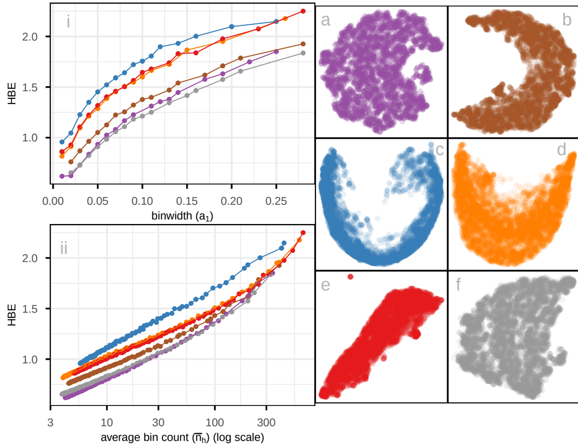
Figure 12: Assessing which of the 6 NLDR layouts of the MNIST digit 1 data is the better representation using HBE for varying (i) binwidth ( a_1 ), and (ii) average bin count ( \bar{n}_h ). Colour is used for the lines and points in the left plot to match the scatterplots of the NLDR layouts (a-f). Layout c is universally poor. Layouts a, f that show a big cluster and a small circular cluster are universally optimal. Layout a performs well at tiny binwidth (where most points are in their own bin) and not as well as f with larger binwidth, thus layout f is the best choice. Plot (ii), which accounts for the density within clusters by using average bin count, shows reduced differences between layouts, indicating that part of the variation in (i) is driven by cluster density rather than true structural differences.
