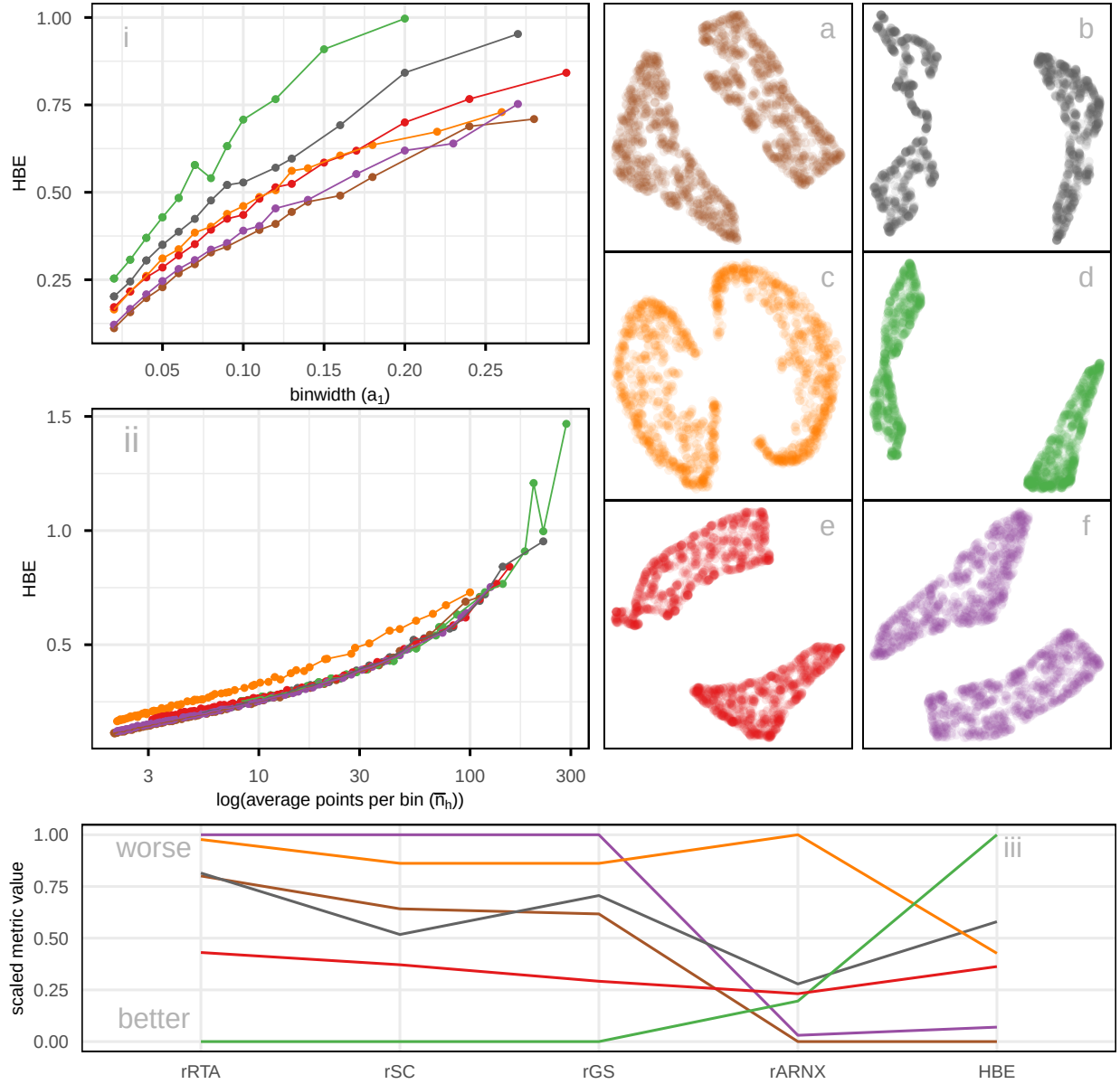
Figure 8: Assessing which of the 6 NLDR layouts (a-f) on the 2NC7 data is the better representation using HBE for varying binwidth ( a_1 ) and average bin count ( \bar{n}_h ). Color represents NLDR layout. Layout d is universally poor. Layouts a, b, e that show two close clusters are universally suboptimal. Layout b with little separation performs well at tiny binwidth (where most points are in their own bin) and poorly as binwidth increases. Layout e has small separation with oddly shaped clusters. Layout a is the best choice. Comparison of scaled evaluation metrics (rRTA, rSC, rGS, rARNX, and HBE using a_1 = 0.05 ) for the six NLDR layouts computed on the 2NC7 data using a parallel coordinate plot. Color of the line indicates NLDR layout. RTA, SC, GS, and ARNX is reversed so that lower is best.
