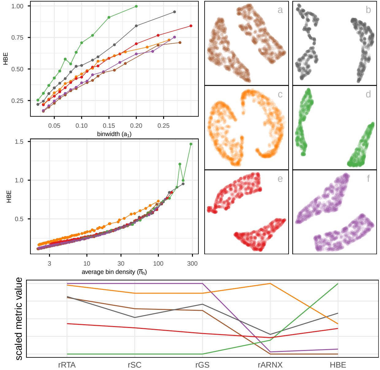
Figure 8: Assessing which of the 6 NLDR layouts (a-f) on the 2NC7 data is the better representation using HBE for varying binwidth ( a_1 ) and average bin density ( \bar{n}_h ). Color represents NLDR layout. Layout d is universally poor. Layouts a, b, e that show two close clusters are universally suboptimal. Layout b with little separation performs well at tiny binwidth (where most points are in their own bin) and poorly as binwidth increases. Layout e has small separation with oddly shaped clusters. Layout a is the best choice. Comparison of scaled evaluation metrics (rRTA, rSC, rGS, rARNX, and HBE using a_1 = 0.05 ) for the six NLDR layouts computed on the 2NC7 data using a parallel coordinate plot. Color of the line indicates NLDR layout. RTA, SC, GS, and ARNX is reversed so that lower is best.
