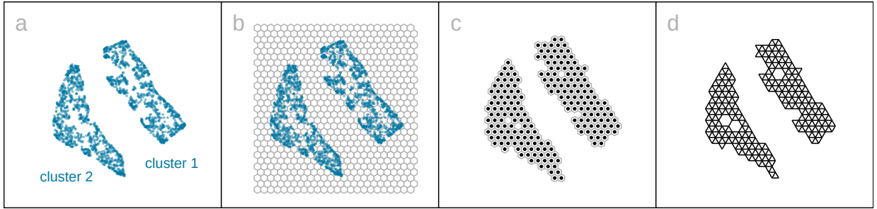
Figure 2: Key steps for constructing the model on the tSNE layout ( k = 2 ): (a) data, (b) hexagon bins, (c) bin centroids, and (d) triangulated centroids. The layout used is a reasonable reprersntation of the 2NC7 data, which contains two curvilinear clusters that have been flattened into a triangular and rectangular shape.
