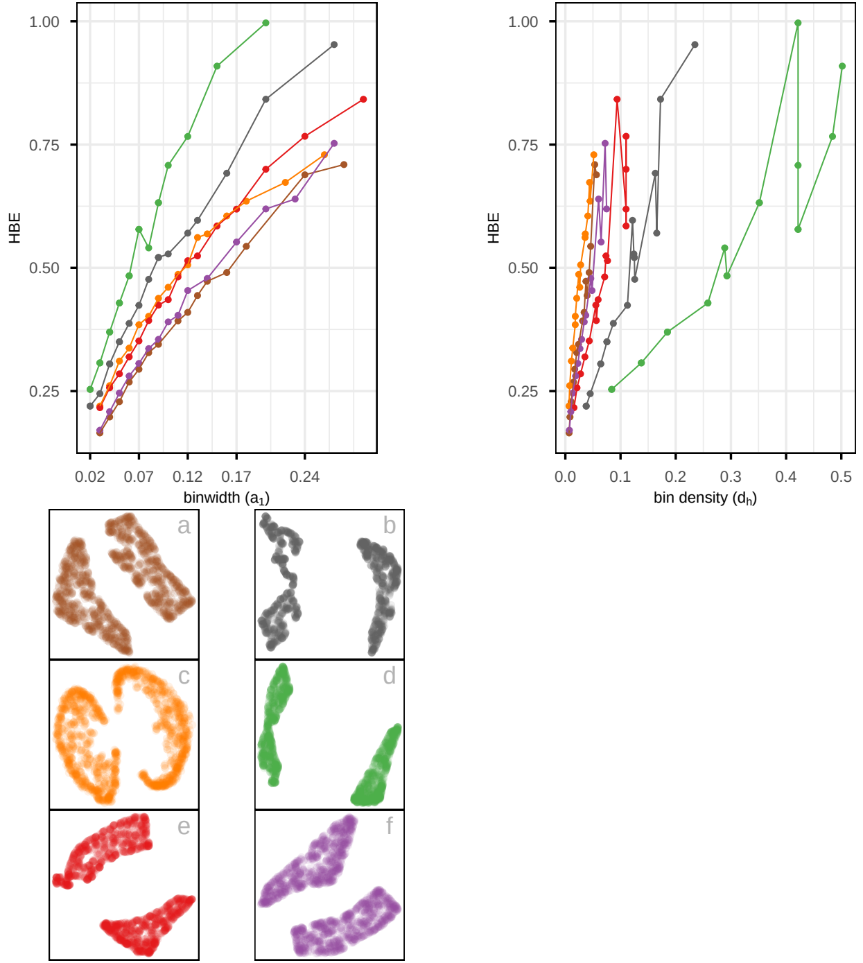
Figure 8: Assessing which of the 6 NLDR layouts on the 2NC7 data is the better representation using HBE for varying binwidth ( a_1 ). Color used for the lines and points in the left plot and in the scatterplots represents NLDR layout (a-f). Layout d is universally poor. Layouts a, b, e that show two close clusters are universally suboptimal. Layout b with little separation performs well at tiny binwidth (where most points are in their own bin) and poorly as binwidth increases. Layout e has small separation with oddly shaped clusters. Layout a is the best choice.
