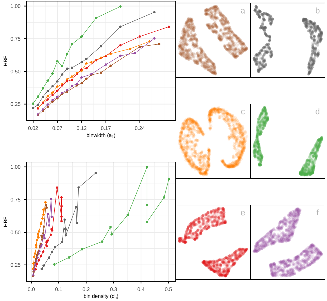
Figure 8: Assessing which of the 6 NLDR layouts on the 2NC7 data is the better representation using HBE for varying binwidth ( a_1 ). Color used for the lines and points in the left plot and in the scatterplots represents NLDR layout (a-f). Layout d is universally poor. Layouts a, b, e that show two close clusters are universally suboptimal. Layout b with little separation performs well at tiny binwidth (where most points are in their own bin) and poorly as binwidth increases. Layout e has small separation with oddly shaped clusters. Layout a is the best choice.
