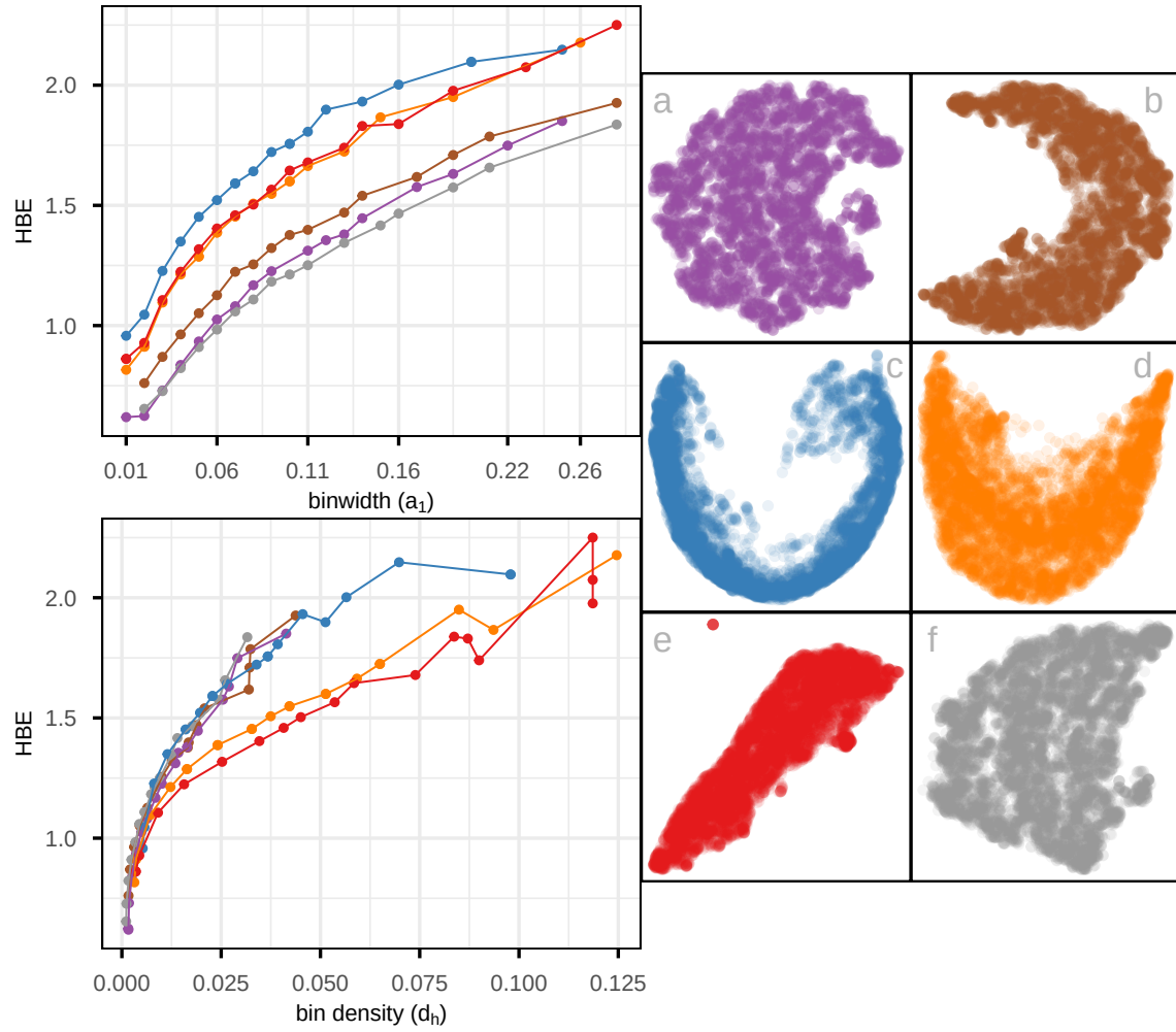
Figure 12: Assessing which of the 6 NLDR layouts of the MNIST digit 1 data is the better representation using HBE for varying binwidth ( a_1 ). Colour is used for the lines and points in the left plot to match the scatterplots of the NLDR layouts (a-f). Layout c is universally poor. Layouts a, f that show a big cluster and a small circular cluster are universally optimal. Layout a performs well at tiny binwidth (where most points are in their own bin) and not as well as f with larger binwidth, thus layout f is the best choice.
