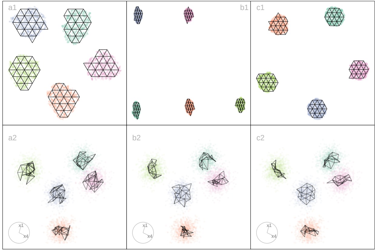
Figure 4: NLDR’s organize points in the 2- D layout in different ways, possibly misleadingly, illustrated using three layouts: (a) tSNE, (b) UMAP, (c) PaCMAP. The data has five Gaussian clusters in 4- D . The bottom row of plots shows a 2- D projection from a tour on 4- D revealing the differences generated by the layouts on the model fits. We would expect the model fit to be like that in (a2) where it is distinctly is separate for each cluster but like a hairball in each. This would indicate the distinct clusters, each being fully 4- D . With (c2), the curiosity is that the model is a 2- D pancake shape in 4- D , indicating that there is some ordering of points done by PaCMAP, possibly along some principal component axes. Videos of the langevitour animations are available at https://youtu.be/I-kxCwVfqiQ , https://youtu.be/gD1P01FUPyU , and https://youtu.be/MxJ_srOFQNk respectively.
