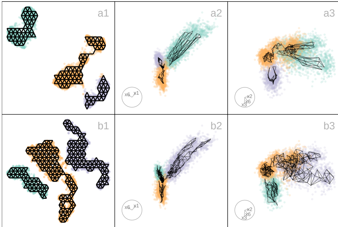
Figure 7: Compare the published 2- D layout (Figure 6 a) made with UMAP and the 2- D layout made with tSNE selected as optimal by scDEED (Figure 6 b) and also HBE (Figure 6). The two plots on the right show projections from a tour, with the models overlaid. The published layout a suggested three separated clusters with two of them are close, but this is not present in the data. While there may be three clusters they are not well-separated. The difference in model fit also indicates this: the published layout a does not capture the nonlinear structure of the clusters like the model generated from layout b. This supports the choice that layout b is the better representation of the data, because it shows close clusters. Videos of the langevitour animations are available at https://youtu.be/ffiB4MGWyn8 and https://youtu.be/e7XNL18co1c respectively.
