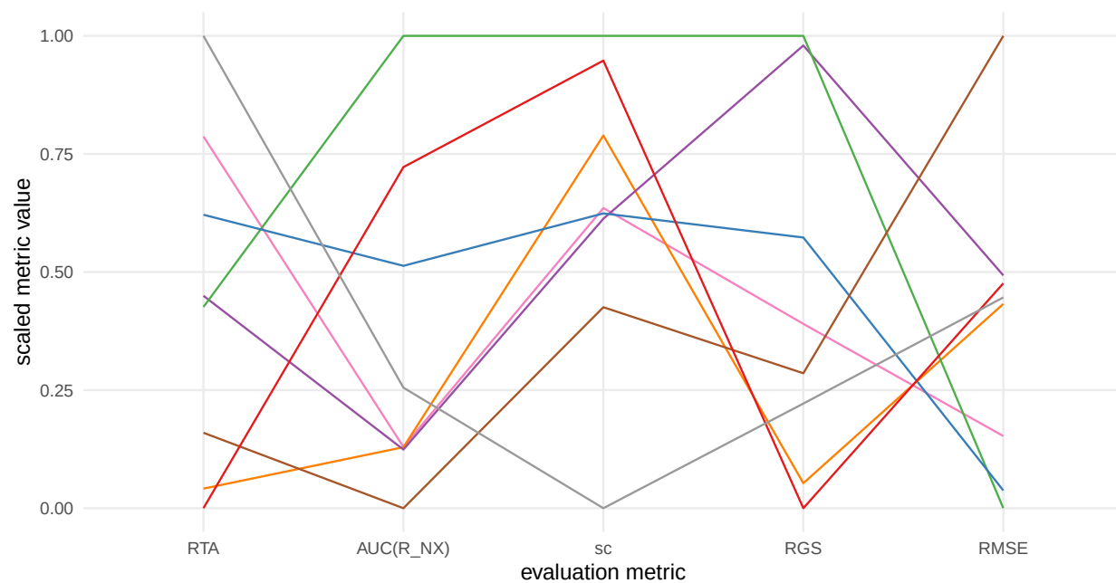
Figure 6: Comparison of evaluation metrics across eight NLDR layouts for the PBMC data. Each line represents a different NLDR layout evaluated using multiple normalized metrics: RTA, AUC(R_NX), sc, RGS, and RMSE. The variation across metrics shows that each captures different aspects of structure preservation, and none behave exactly like RMSE. RTA shows a somewhat similar ordering across methods.
