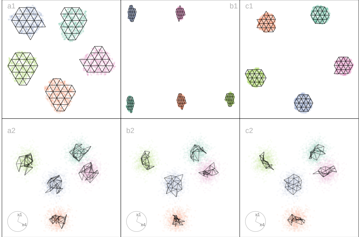
Figure 10: NLDL's organise points in the 2- D layout in different ways, possibly misleadingly, illustrated using three layouts: (a) tSNE, (b) UMAP, (c) PaCMAP. The data has five Gaussian clusters in 4- D . The bottom row of plots shows a 2- D projection from a tour on 4- D revealing the differences generated by the layouts on the model fits. We would expect the model fit to be like that in (a2) where it is distinctly is separate for each cluster but like a hairball in each. This would indicate the distinct clusters, each being fully 4- D . With (c2), the curiosity is that the model is a 2- D pancake shape in 4- D , indicating that there is some ordering of points done by PaCMAP, possibly along some principal component axes.
