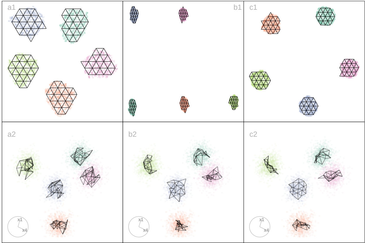
Figure 6: NLDL's organize points in the 2- D layout in different ways, possibly misleadingly, illustrated using three layouts: (a) tSNE, (b) UMAP, (c) PaCMAP. The data has five Gaussian clusters in 4- D . The bottom row of plots shows a 2- D projection from a tour on 4- D revealing the differences generated by the layouts on the model fits. We would expect the model fit to be like that in (a2) where it is distinctly is separate for each cluster but like a hairball in each. This would indicate the distinct clusters, each being fully 4- D . With (c2), the curiosity is that the model is a 2- D pancake shape in 4- D , indicating that there is some ordering of points done by PaCMAP, possibly along some principal component axes. Videos of the langevitour animations are available at https://youtu.be/I-kxCwVfqiQ , https://youtu.be/gD1P01FUPyU , and https://youtu.be/MxJ_srOFQNk respectively.
