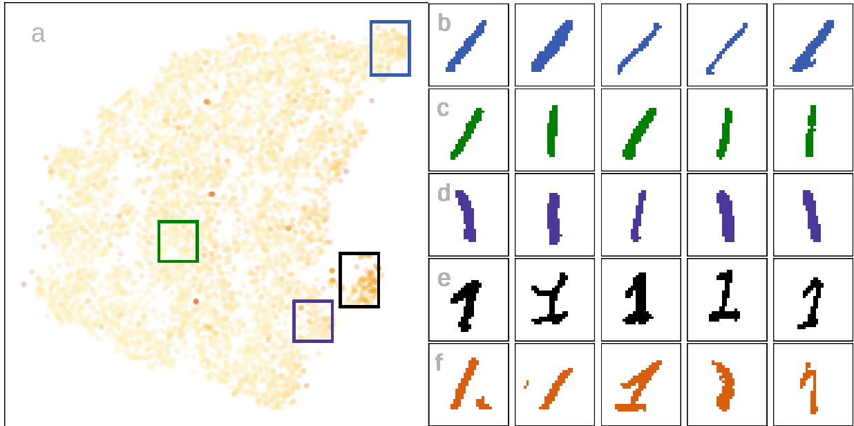
Figure 14: There is a pattern to error of the fit of the model for 2- D layout of the MNIST digit 1 data. On the left is the NLDR layout (a), and at right (b-e) are images of samples of observations taken at locations along the big cluster, and the small cluster, showing how the 1's were drawn. Set (f) are images corresponding to large residuals in the big cluster. Along the big cluster, the angle of digit 1 changes (b-d). The small cluster has larger residuals, and the images show that these tend to be European style with a flag at the top, and a base at the bottom. The set in (f) show various poorly written digits.
