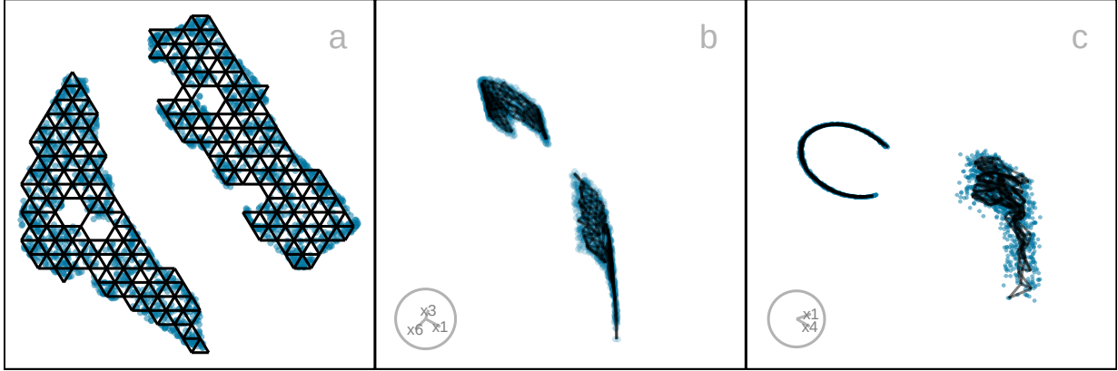
Figure 4: Lifting the 2-D fitted model into p -D. Two projections of the p -D fitted model overlaying the data are shown in b, c. The fit is reasonably tight with the data in one cluster (top one in b), but slightly less so in the other cluster probably because it is 3-D. Notice also that, in the 2-D layout the two clusters have internal gaps which creates a model with some holes. This lacy pattern happens regardless of the hyper-parameter choice, but this doesn't severely impact the p -D model representation.
