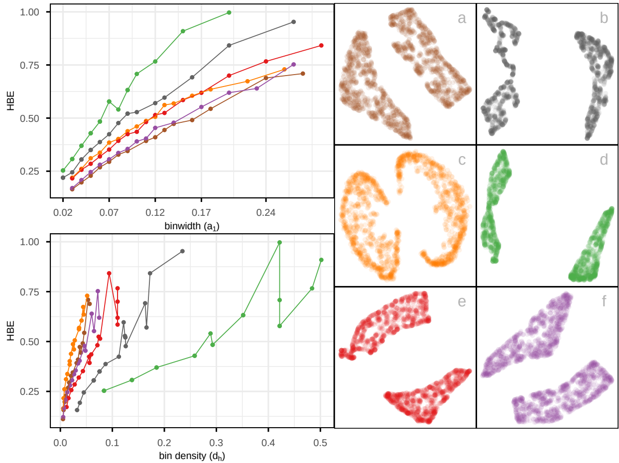
Figure 8: Assessing which of the 6 NLDR layouts on the 2NC7 data is the better representation using HBE for varying binwidth ( a_1 ). Color used for the lines and points in the left plot and in the scatterplots represents NLDR layout (a-f). Layout d is universally poor. Layouts a, b, e that show two close clusters are universally suboptimal. Layout b with little separation performs well at tiny binwidth (where most points are in their own bin) and poorly as binwidth increases. Layout e has small separation with oddly shaped clusters. Layout a is the best choice.
