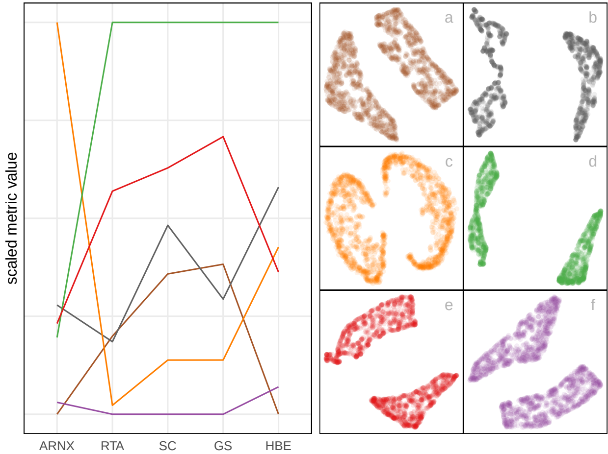
Figure 9: Comparison of scaled evaluation metrics (ARNX, RTA, SC, GS, and HBE using a_1 = 0.05 ) for the six NLDR layouts computed on the 2NC7 data using a parallel coordinate plot. Color of the line indicates NLDR layout. ARNX is reversed so that lower is best. RTA, SC and GS should be reversed, too, but they best match ARNX and HBE without doing so! There is some general agreement, and small disagreements, with ARNX being most different. All agree that layout f is good, and almost all that d is bad. Interestingly, there is disagreement on layout a, which is almost the same as layout f.
