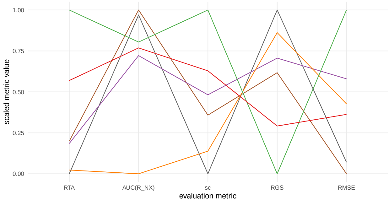
Figure 9: Comparison of scaled evaluation metrics across NLDR representations. Each line represents a different layout evaluated using multiple metrics RTA, \text{AUC}(\text{R\_NX}) , sc, RGS, and RMSE. The variability across metrics highlights that no single measure universally captures embedding quality, underscoring the importance of considering multiple diagnostics when assessing representation faithfulness.
