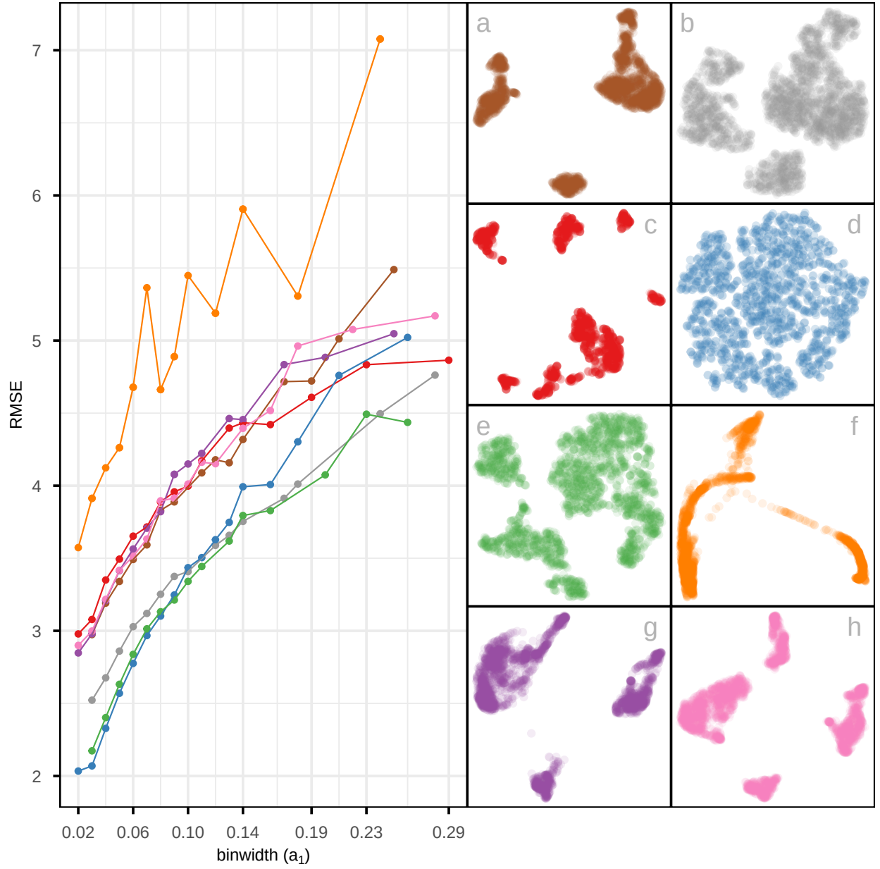
Figure 10: Assessing which of the 8 NLDR layouts on the PBMC3k data (shown in Figure 1) is the better representation using RMSE for varying binwidth ( a_1 ). Color used for the lines and points in the left plot and in the scatterplots represents NLDR layout (a-h). Layout f is universally poor. Layouts a, c, g, h that show large separations between clusters are universally suboptimal. Layout d with little separation performs well at tiny binwidth (where most points are in their own bin) and poorly as binwidth increases. The choice of best is between layouts b and e, that have small separations between oddly shaped clusters. Layout e is chosen as the best.
