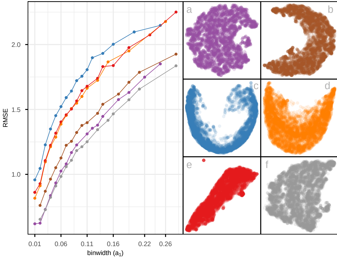
Figure 12: Assessing which of the 6 NLDR layouts of the MNIST digit 1 data is the better representation using RMSE for varying binwidth ( a_1 ). Colour is used for the lines and points in the left plot to match the scatterplots of the NLDR layouts (a-f). Layout c is universally poor. Layouts a, f that show a big cluster and a small circular cluster are universally optimal. Layout a performs well at tiny binwidth (where most points are in their own bin) and not as well as f with larger binwidth, thus layout f is the best choice.
