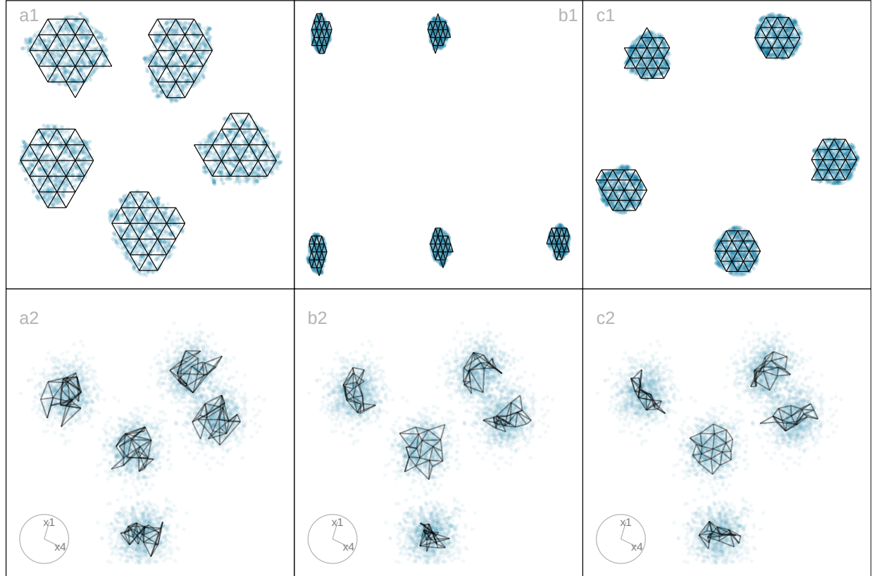
Figure 8: NLDR's organise points in the 2- D layout in different ways, possibly misleadingly, illustrated using three layouts: (a) tSNE, (b) UMAP, (c) PaCMAP. The data has five Gaussian clusters in 4- D . The bottom row of plots shows a 2- D projection from a tour on 4- D revealing the differences generated by the layouts on the model fits. We would expect the model fit to be like that in (a2) where it is distinctly is separate for each cluster but like a hairball in each. This would indicate the distinct clusters, each being fully 4- D . With (c2), the curiosity is that the model is a 2- D pancake shape in 4- D , indicating that there is some ordering of points done by PaCMAP, possibly along some principal component axes.
