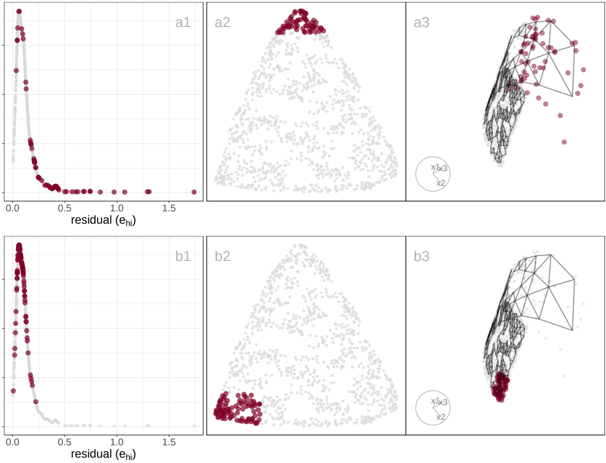
Figure 9: Exploring the effect of density on the NLDR layout using a 2- D curved sheet in 4- D with different density at each end. Three plots are linked: density plot of residuals (a1, b1), NLDR layout (a2, b2), projection of 4- D model and data (a3, b3). The brown points indicate the selected set, which are different in each row. In (a2), the top part of the triangular shape is selected which corresponds to higher residuals (a1) and the sparse end of the structure (a3). In (b2) one of other corners is highlighted, which can be seen to correspond to low residuals (b1) and one side of the dense end of the data (b3). While the tSNE layout represents the dense end of the sheet correctly as two corners in the layout, it contracts the sparse end of the sheet into a single corner.
