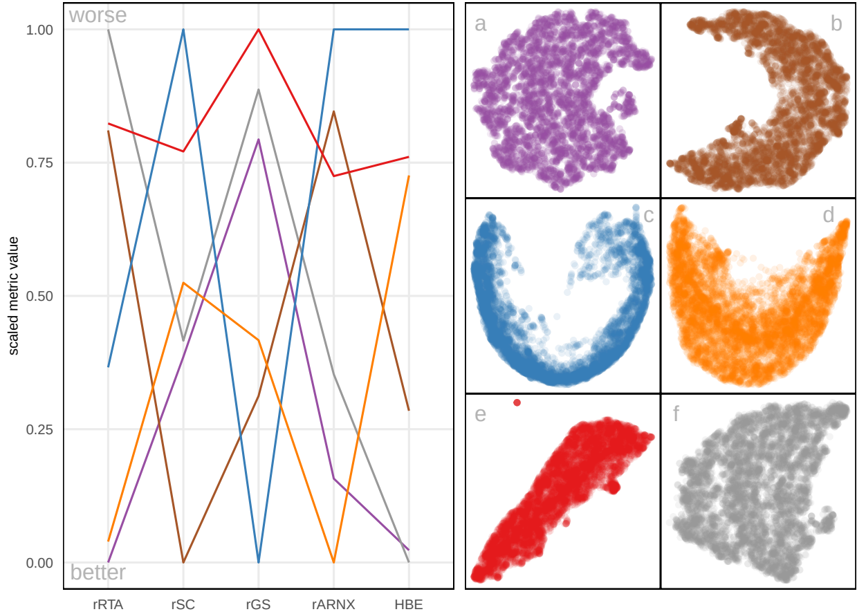
Figure 9: Comparison of scaled evaluation metrics (rARNX, rRTA, rSC, rGS, and HBE using a_1 = 0.04 ) for six NLDR layouts computed on the MNIST digit 1 data using a parallel coordinate plot. Each line represents a layout (a–f), with colors corresponding to the scatterplots shown on the right. The metrics display different ranking patterns, indicating that no single measure fully captures embedding quality. Layout a is identified as the best according to HBE and rRTA, but is considered much less optimal by rARNX, rSC, and rGS. Layout e is considered the worst, or close to the poorest, by all metrics. Layouts a and f show similar patterns of agreement across metrics, except for rRTA, where layout a performs the best and layout f the worst. Layout c is the worst in rARNX, rSC, and HBE.
