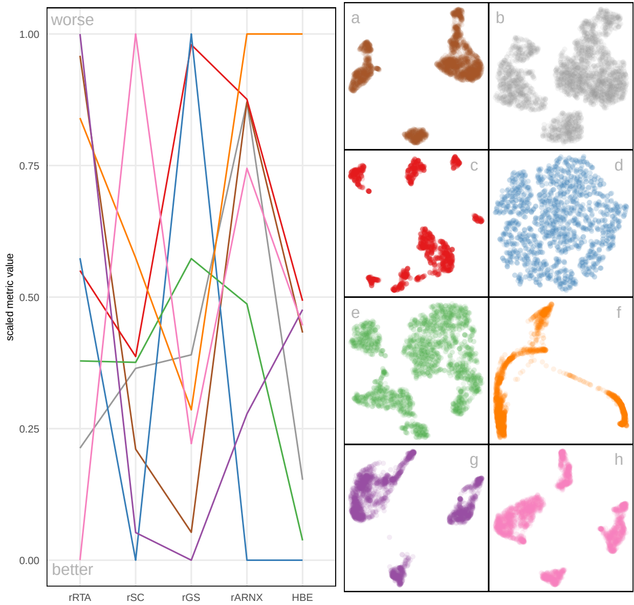
Figure 8: Comparison of scaled evaluation metrics (rRTA, rSC, rGS, rARNX, and HBE with a_1 = 0.06 ) for the eight NLDR layouts computed on the PBMC3k data, shown as a parallel coordinate plot. The color of each line corresponds to a NLDR layout. All, except rGS and rARNX agree that layout e is best or very close to best. Layout d is best according to HBE and rARNX but considered to be much less optimal by rRTA, rSC and rGS. Layout f is considered poor by rARNX and HBE. Layout a is considered close to the best by rGS and rSC.
