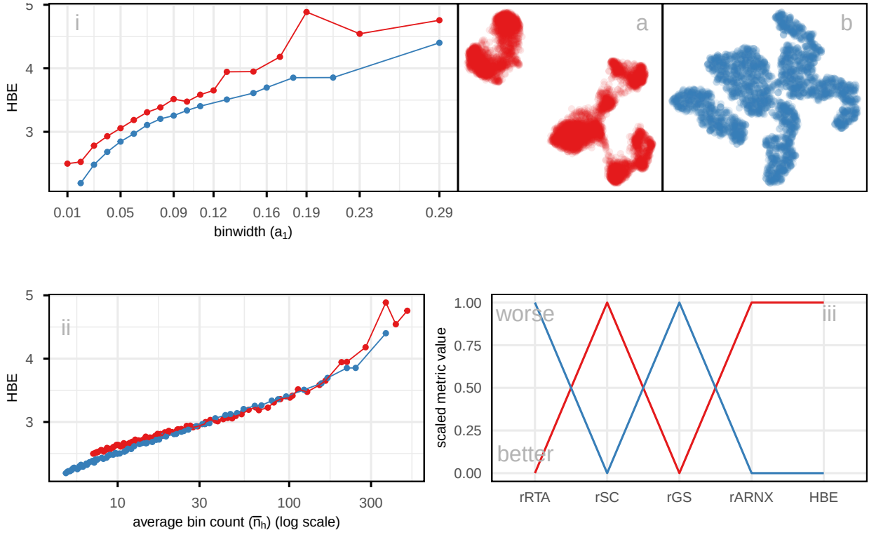
Figure 6: Comparing the published layout (a) with what would be suggested to be optimal by scDEED (b), using HBE for varying (i) binwidth ( a_1 ), and (ii) average bin count ( \bar{n}_h ), on a subset of PBMC3k data. Color represents NLDR layouts. HBE would corroborate that the scDEED optimised layout is better than what was originally published. Plot (ii), which accounts for the density within clusters by using average bin count, shows reduced differences between layouts, indicating that part of the variation in (i) is driven by cluster density rather than true structural differences. Comparison of scaled evaluation metrics (iii) (rRTA, rSC, rGS, rARNX, and HBE using a_1 = 0.04 ) for two NLDR layouts of the PBMC3k data the originally published layout (a) and the scDEED optimised layout (b). Each line represents a layout, with color matching the corresponding scatterplots. Most metrics (rSC, rARNX, and HBE) consistently indicate that the optimised layout (b) provides a better representation, while rRTA, and rGS slightly favor the published layout.
