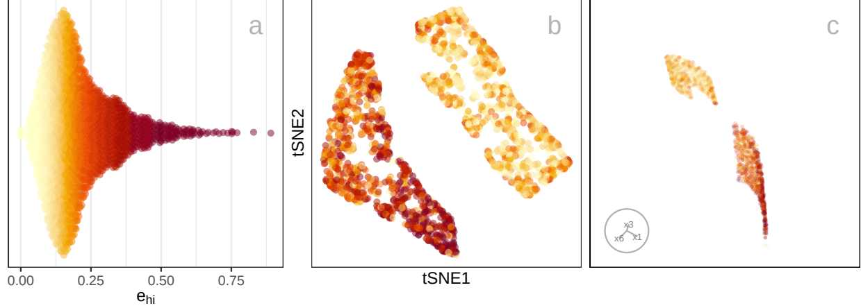
Figure 5: Examining the distribution of residuals in a jittered dotplot (a), 2- D NLDR layout (b) and a tour of 4- D data space (c). Color indicates residual ( e_{hi} ), dark color indicating high value. Most large residuals are distributed in one cluster (bottom one in c) and most small residuals are distributed in the other cluster.
