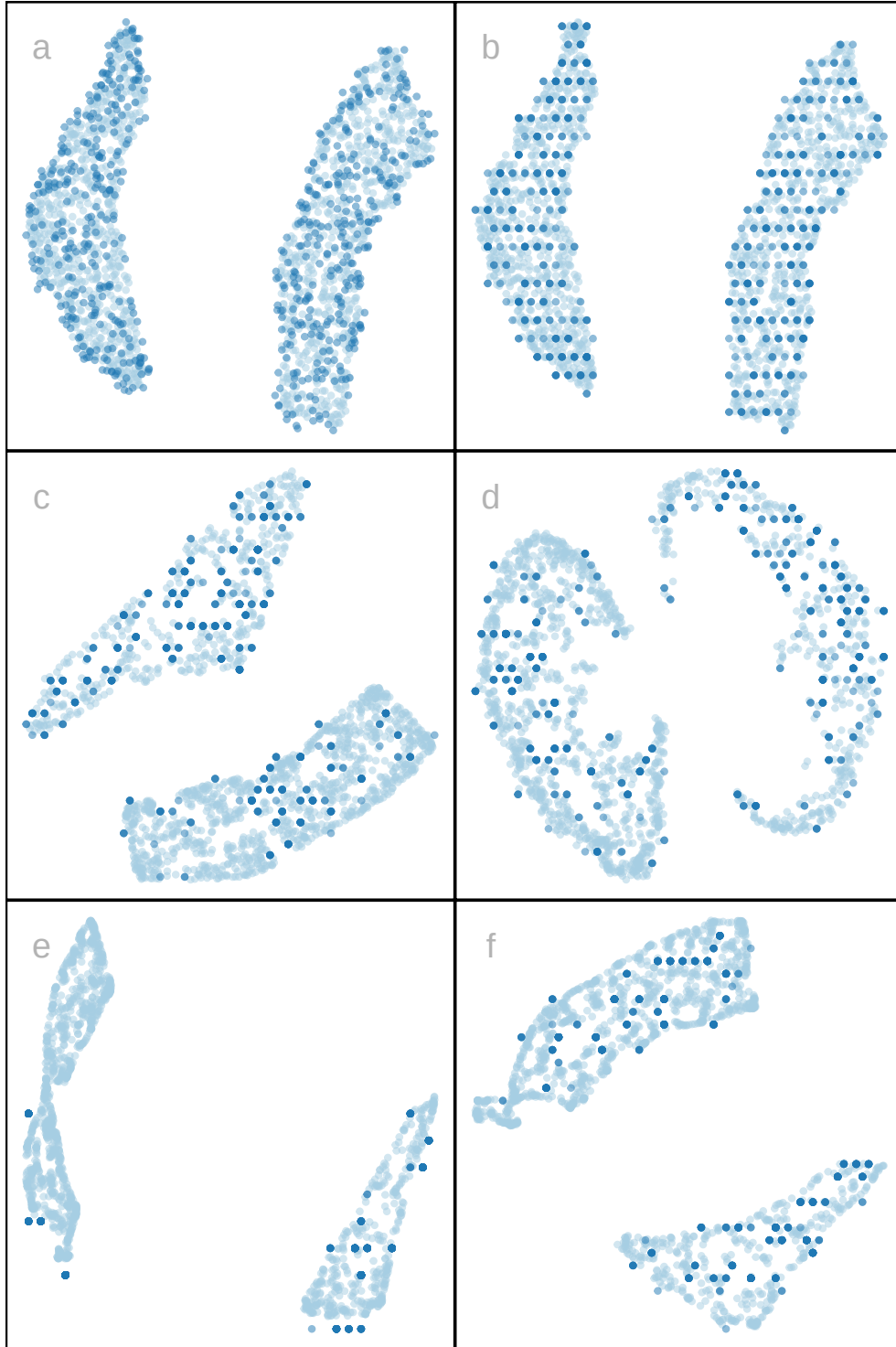
Figure 7: Comparison of predictions made by UMAP and by our method, relative to the training data. Dark points are the predicted test set, and lighter points are the training sample used to create the layouts. Panel (a) shows predictions obtained using the UMAP predict() function. Panels (b)–(f) show predictions obtained using our method applied to (b) UMAP, (c) tSNE, (d) PHATE, (e) TriMAP, and (f) PaCMAP layouts, respectively.
