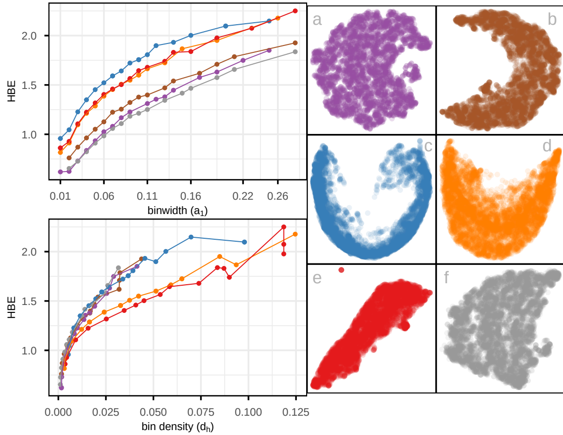
Figure 11: Assessing which of the 6 NLDR layouts of the MNIST digit 1 data is the better representation using HBE for varying binwidth ( a_1 ). Colour is used for the lines and points in the left plot to match the scatterplots of the NLDR layouts (a-f). Layout c is universally poor. Layouts a, f that show a big cluster and a small circular cluster are universally optimal. Layout a performs well at tiny binwidth (where most points are in their own bin) and not as well as f with larger binwidth, thus layout f is the best choice.
