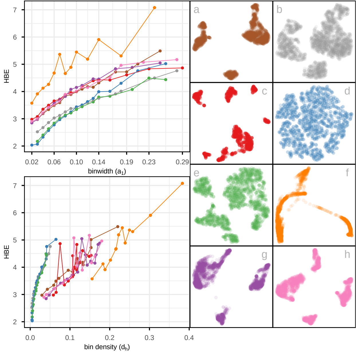
Figure 9: Assessing which of the 8 NLDR layouts on the PBMC3k data (shown in Figure 1) is the better representation using HBE for varying binwidth ( a_1 ). Color used for the lines and points in the left plot and in the scatterplots represents NLDR layout (a-h). Layout f is universally poor. Layouts a, c, g, h that show large separations between clusters are universally suboptimal. Layout d with little separation performs well at tiny binwidth (where most points are in their own bin) and poorly as binwidth increases. The choice of best is between layouts b and e, that have small separations between oddly shaped clusters. Layout e is chosen as the best.
