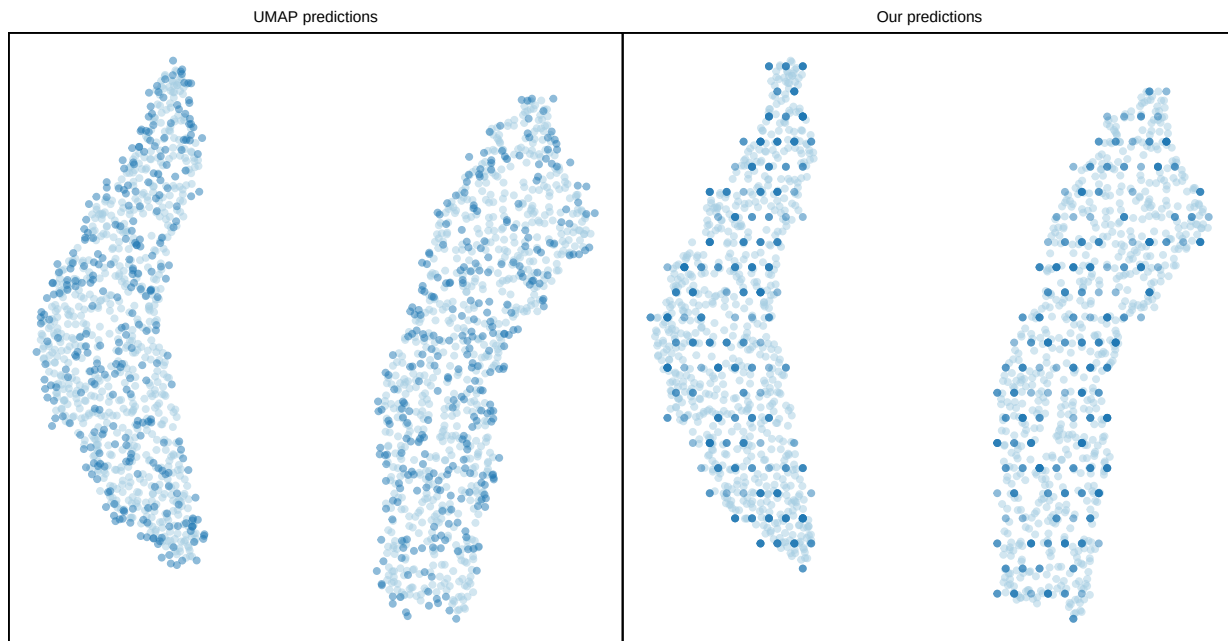
Figure 6: Comparison of predictions made by UMAP and by our method, relative to the training data. Dark points are the predicted test set, and lighter points are the training sample used to create the UMAP layout.
