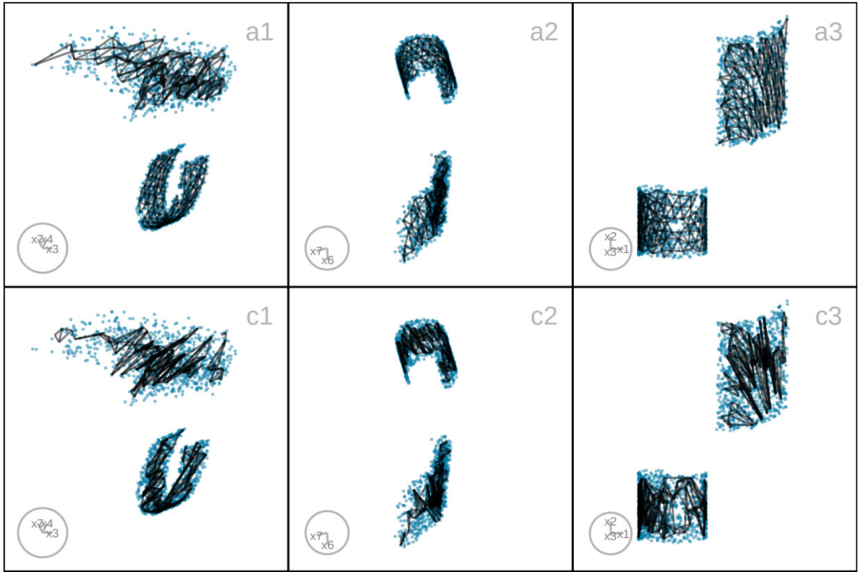
Figure 9: Comparison of fitted models for layouts a and c. Three 2- D projections are shown with fitted model overlaying the 2NC7 data. Layout a (top row) preserves the true nonlinear structure. In contrast, layout c (bottom row) squeezes the model and fails to capture the full width of the underlying shapes. By visualizing the model-in-data space is important to identify these quirks and layout a provides a more faithful representation than layout c.
