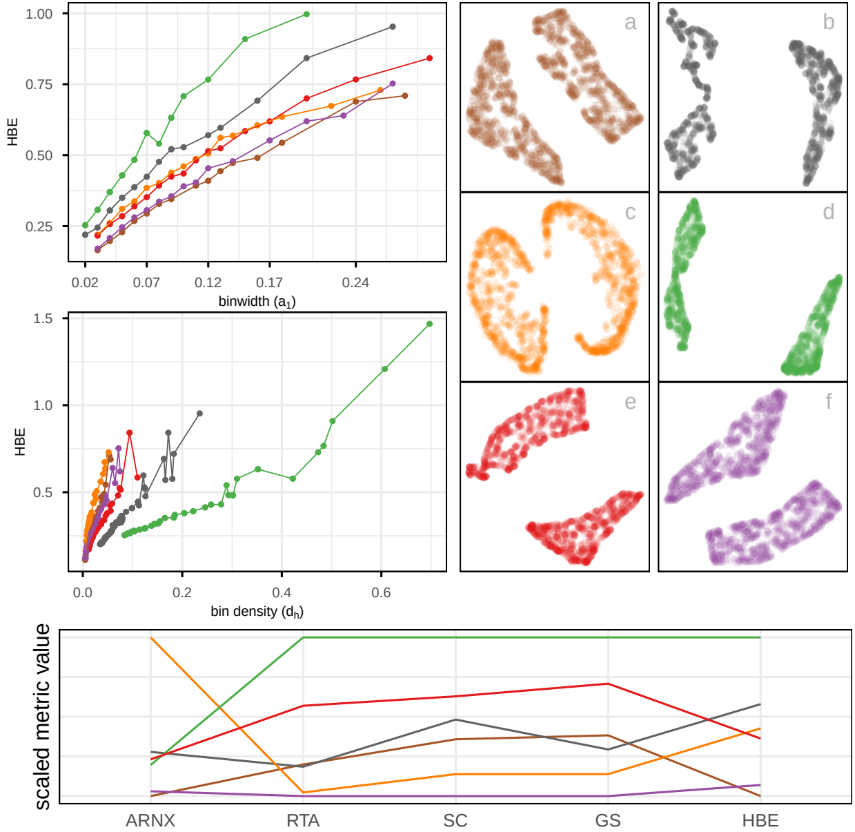
Figure 8: Assessing which of the 6 NLDR layouts on the 2NC7 data is the better representation using HBE for varying binwidth ( a_1 ). Color used for the lines and points in the left plot and in the scatterplots represents NLDR layout (a-f). Layout d is universally poor. Layouts a, b, e that show two close clusters are universally suboptimal. Layout b with little separation performs well at tiny binwidth (where most points are in their own bin) and poorly as binwidth increases. Layout e has small separation with oddly shaped clusters. Layout a is the best choice. Comparison of scaled evaluation metrics (ARNX, RTA, SC, GS, and HBE using a_1 = 0.05 ) for the six NLDR layouts computed on the 2NC7 data using a parallel coordinate plot. Color of the line indicates NLDR layout. ARNX is reversed so that lower is best. RTA, SC and GS should be reversed, too, but they best match ARNX and HBE without doing so! There is some general agreement, and small disagreements, with ARNX being most different. All agree that layout f is good, and almost all that d is bad. Interestingly, there is disagreement on layout a, which is almost the same as layout f.
