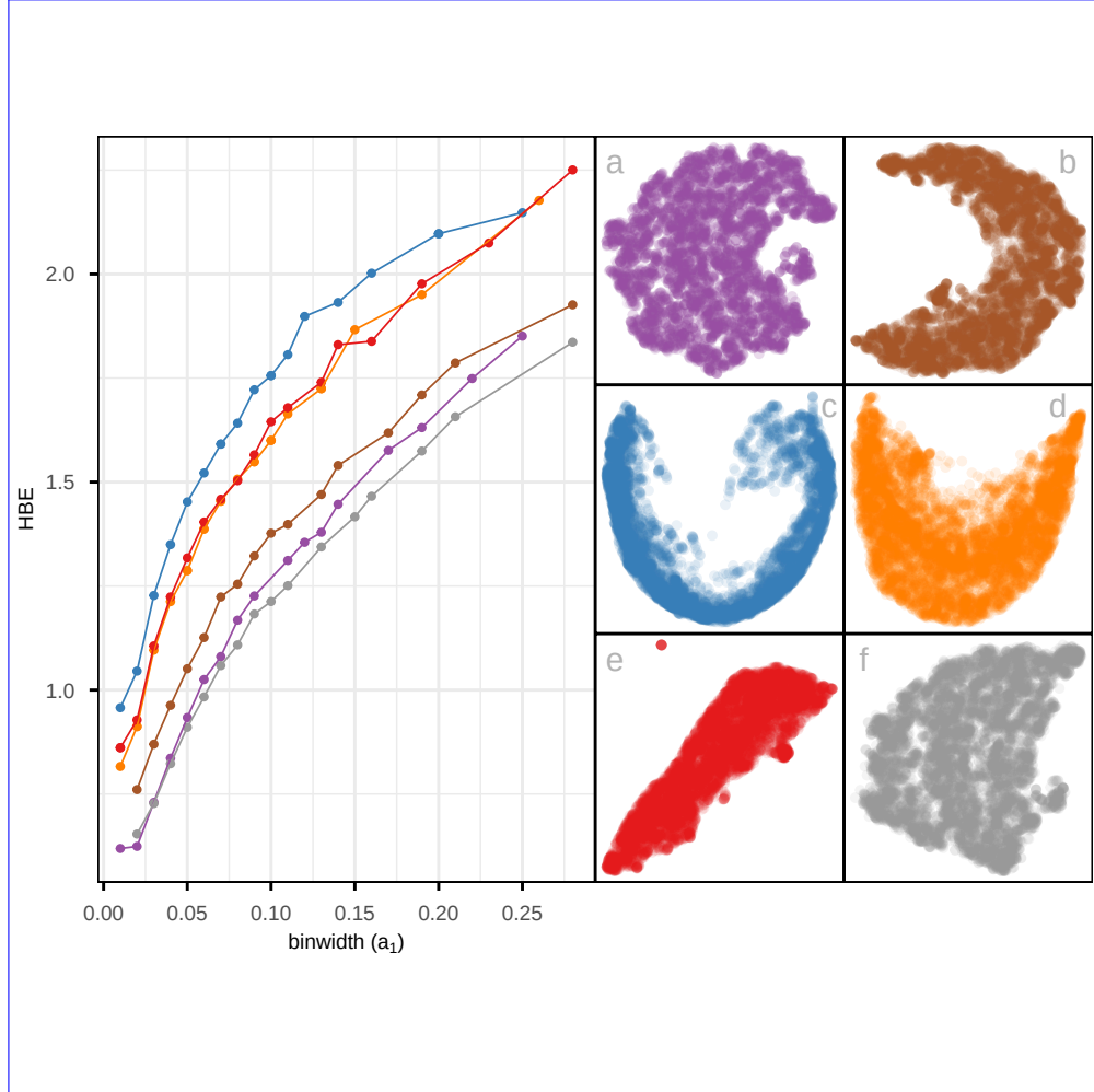
Figure 10: Assessing which of the 6 NLDR layouts of the MNIST digit 1 data is the better representation using HBE for varying (i) binwidth ( a_1 ), and (ii) average bin count ( \bar{n}_h ). Colour Color is used for the lines and points in the left plot to match the scatterplots of the NLDR layouts (a-f). Layout c is universally poor. Layouts a ; and f that show a big cluster and a small circular cluster are universally optimal. Layout a performs well at tiny binwidth (where most points are in their own bin) and not as well as f with larger binwidth, thus layout f is the best choice. Plot (ii), which accounts for the density within clusters by using average bin count, shows reduced differences between layouts, indicating that part of the variation in (i) is driven by cluster density rather than true structural differences.
