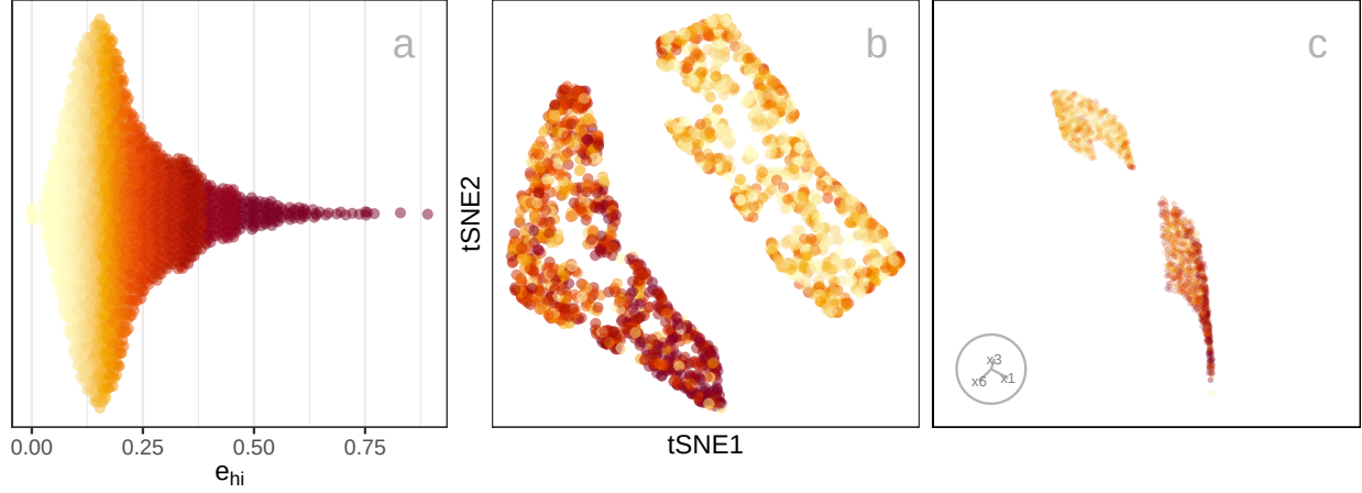
Figure 4: Examining the distribution of residuals in a jittered dotplot (a), 2- D NLDR layout (b) and a tour of 4- D data space (c). Color indicates residual ( e_{hi} ), dark color indicating high value. Most large residuals are distributed in one cluster (bottom one in c) and most small residuals are distributed in the other cluster.
