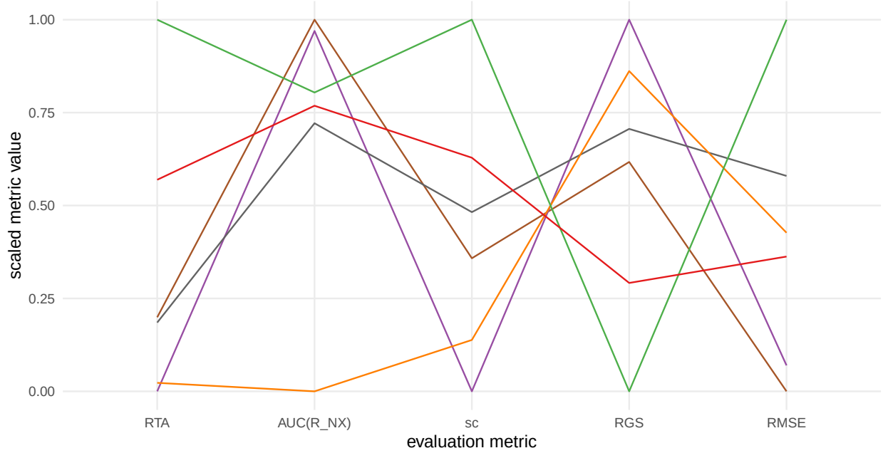
Figure 9: Comparison of scaled evaluation metrics across NLDR representations. Each line represents a different NLDR layout evaluated using multiple normalized metrics: RTA, AUC(R_NX), sc, RGS, and RMSE. The variation across metrics shows that each captures different aspects of structure preservation, and none behave exactly like RMSE. RTA, and sc show a somewhat similar ordering across methods.
