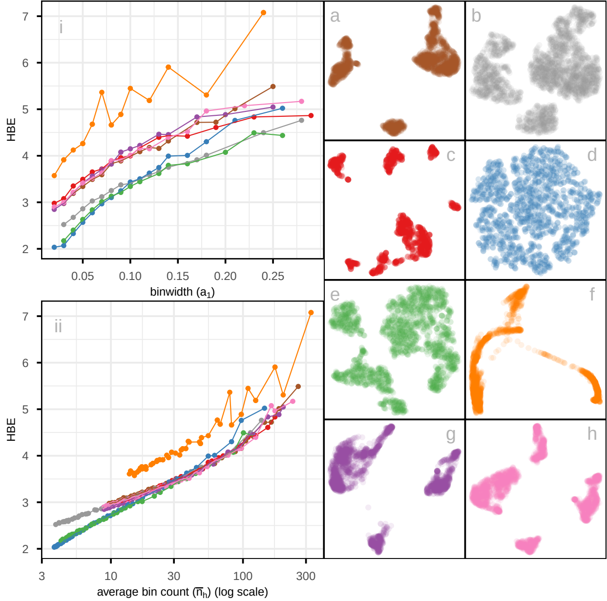
Figure 12: Assessing which of the 8 NLDR layouts on the PBMC3k data is the better representation using HBE for varying (i) binwidth ( a_1 ), and (ii) average bin count ( \bar{n}_h ). Color used for the lines and points in the left plot and in the scatterplots represents NLDR layout (a-h). Layout f is universally poor. Layouts a, c, g, and h that show large separations between clusters are universally suboptimal. Layout d with little separation performs well at tiny binwidth (where most points are in their own bin) and poorly as binwidth increases. The choice of the best is between layouts b and e, which have small separations between oddly shaped clusters. Layout e is chosen as the best. Plot (ii), which accounts for the density within clusters by using average bin count, shows reduced differences between layouts, indicating that part of the variation in (i) is driven by cluster density rather than true structural differences.
