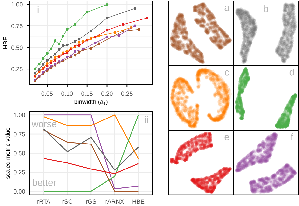
Figure 7: Assessing which of the 6 NLDR layouts (a-f) on the 2NC7 data is the better representation using (i) HBE for varying binwidth ( a_1 ), and (ii) scaled evaluation metrics (rRTA, rSC, rGS, rARNX, and HBE using a_1 = 0.05 ). Color represents the NLDR layout. Using HBE (i), layouts a and f are nearly indistinguishable from each other but have universally lower values than the others: either layout could adequately represent the data. HBE mostly agrees with rARNX, except for layout d. The other metrics rank the layouts in reverse order! The problem though is that they favor more separation, which is misleading for this data. This can be validated by viewing the data in a tour.
