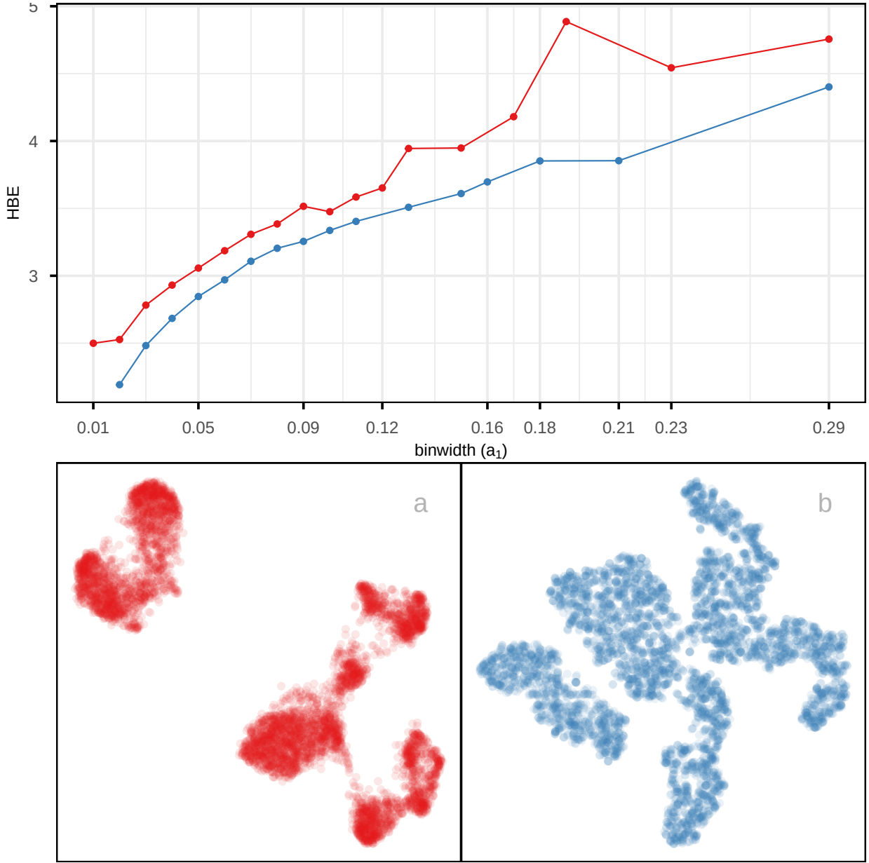
Figure 6: Comparing the published layout (a) with what would be suggested to be optimal by scDEED (b), using HBE vs a_1 , on a subset of PBMC3k data. Color represents NLDR layouts. HBE would corroborate that the scDEED optimised layout is better than what was originally published.
