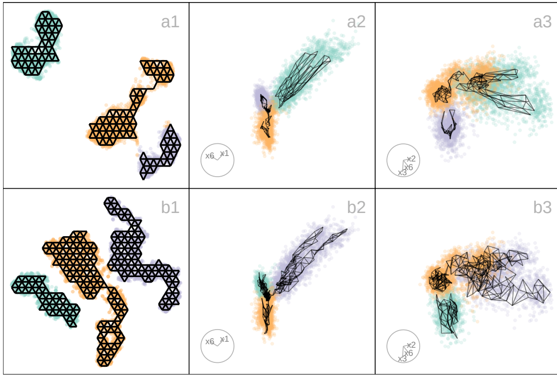
Figure 7: Compare the published 2- D layout (Figure 6 a) made with UMAP and the 2- D layout made with tSNE selected as optimal by scDEED and also HBE (Figure 6 b)(Figure 6). The two plots on the right show projections from a tour, with the models overlaid. The published layout a suggested three separated clusters with two of them are close, but this is not present in the data. While there may be three clusters they are not well-separated. The difference in model fit also indicates this: the published layout a does not capture the nonlinear structure of the clusters like the model generated from layout b. This supports the choice that layout b is the better representation of the data, because it shows close clusters. Videos of the langevitour animations are available at https://youtu.be/ffiB4MGWyn8 and https://youtu.be/e7XNL18co1c respectively.
