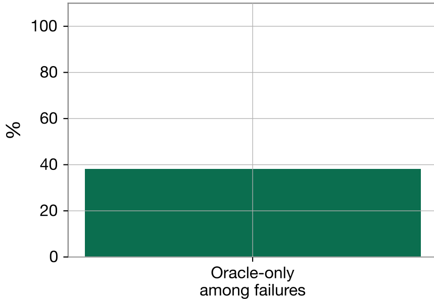
Real GW170817 stress failures (n=34)
