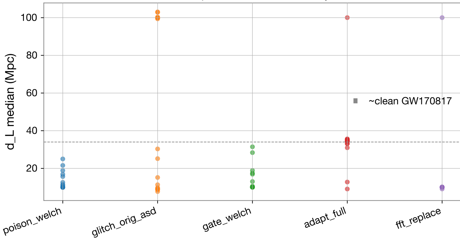
Ablation: per-cell d_L medians by arm
