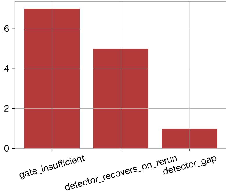
Synthetic failure classes (n=13)
