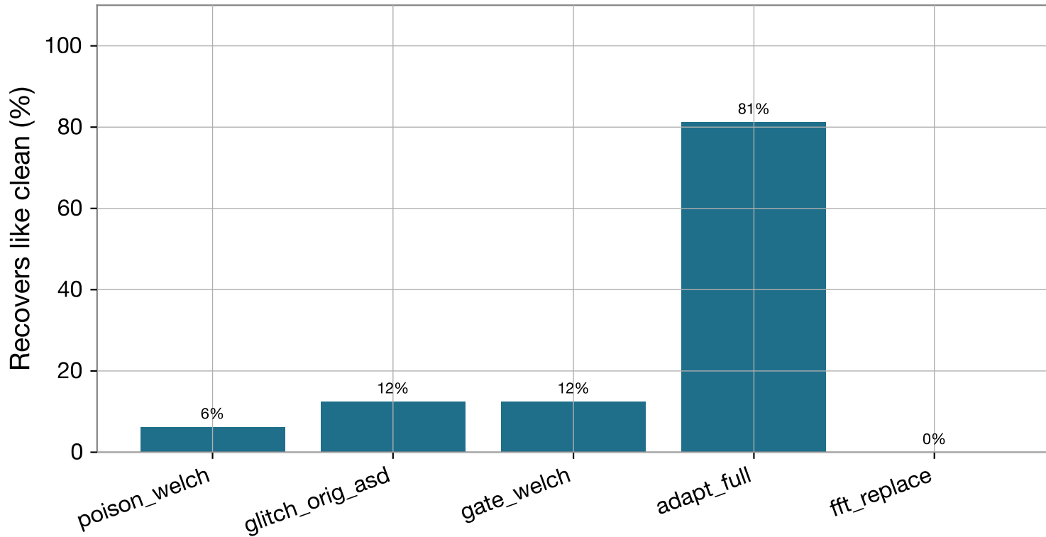
Ablation: recovery rate by arm (16 GW170817 cells)
