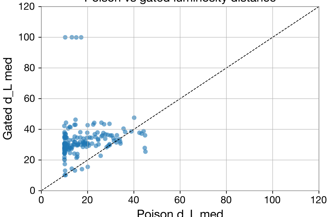
Poison vs gated luminosity distance
