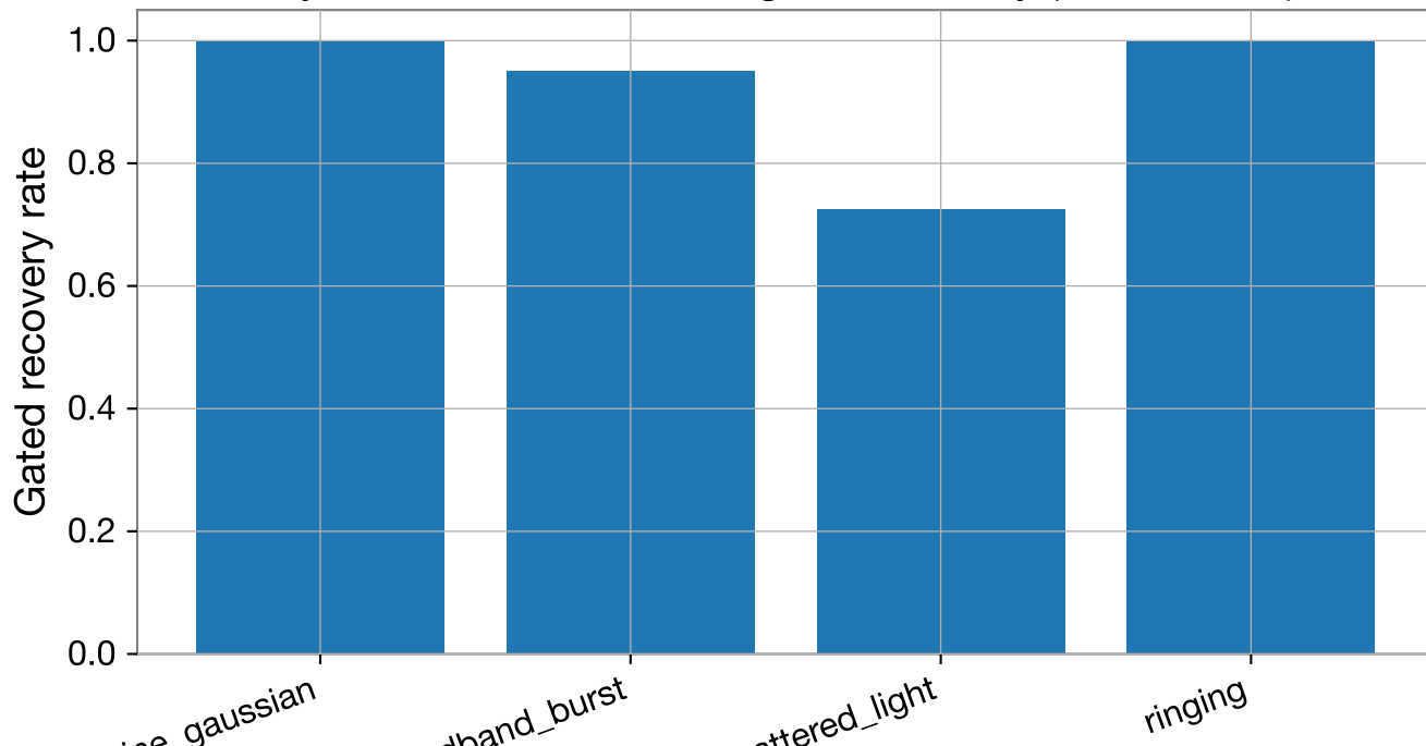
Synthetic BNS ADAPT — gated recovery (overall=0.92)
