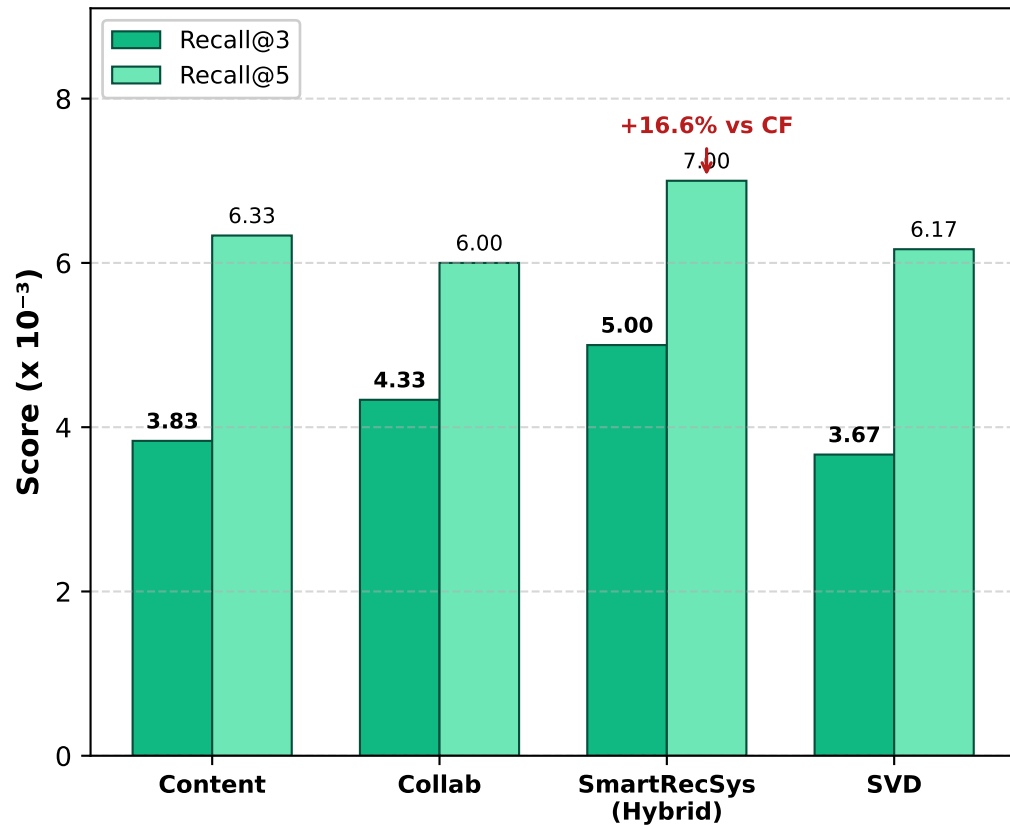
(b) Recall Benchmark (R@3 & R@5)
