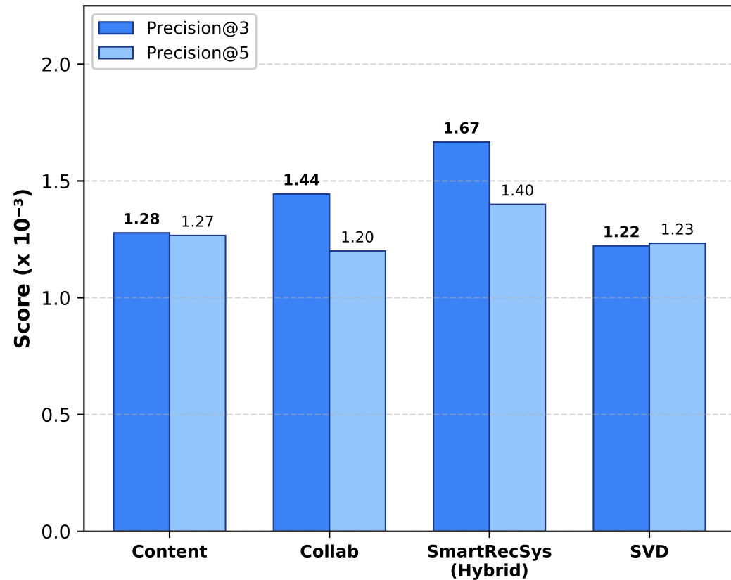
(a) Precision Benchmark (P@3 & P@5)
