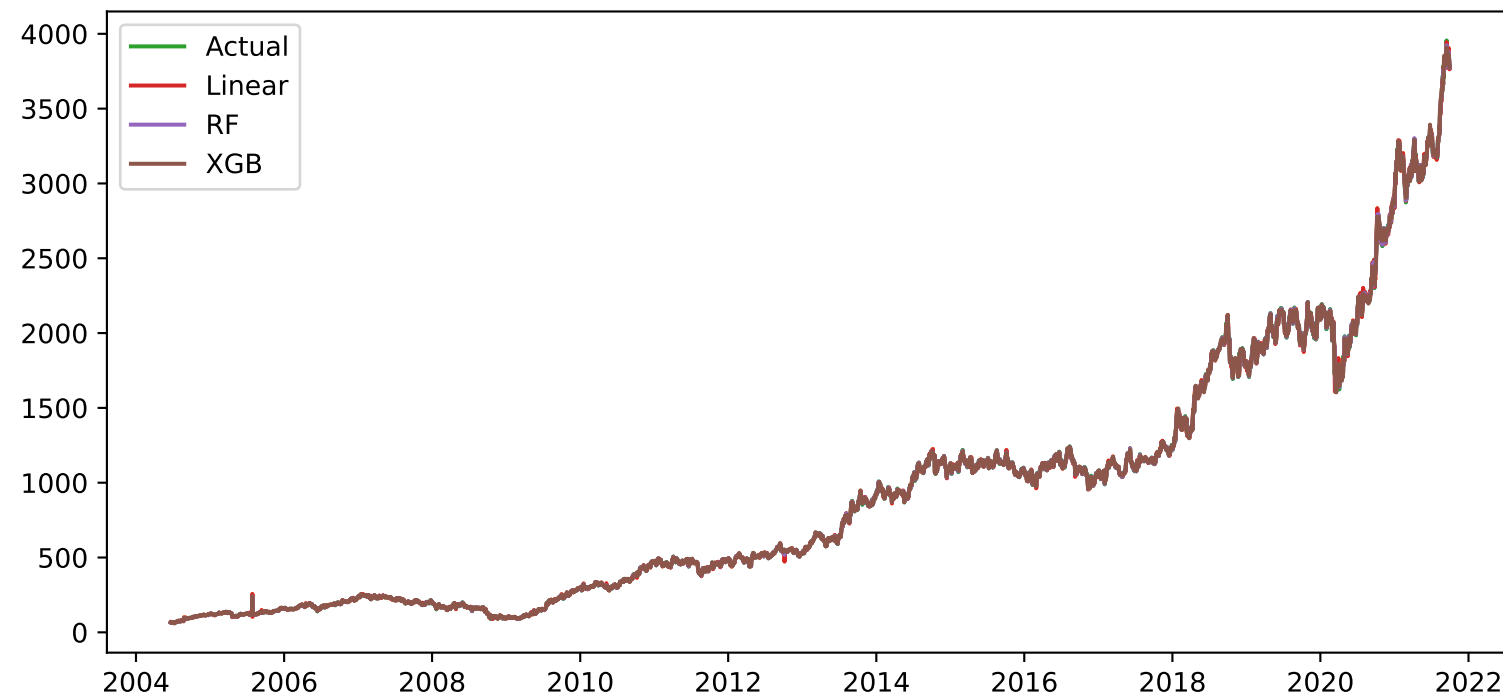
Model Predictions
