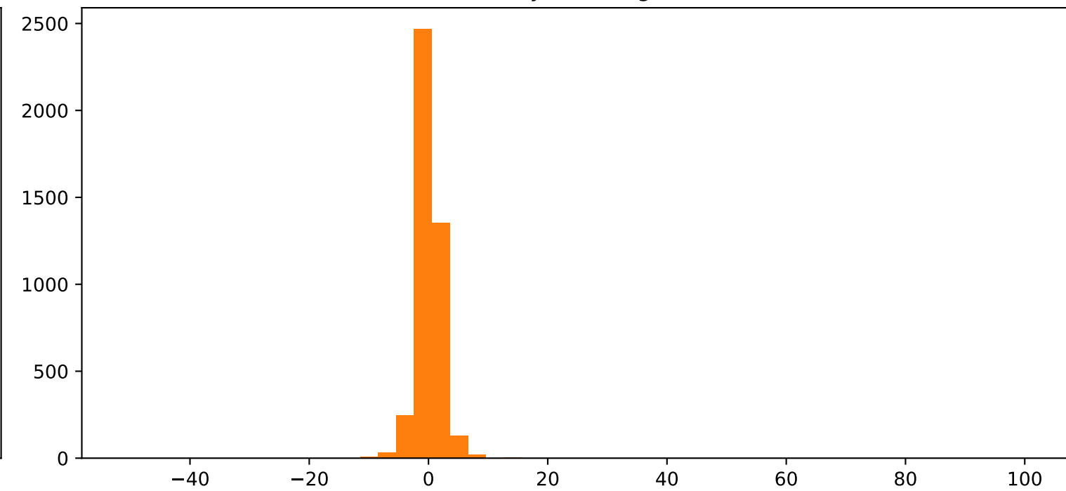
LSTM Forecast
