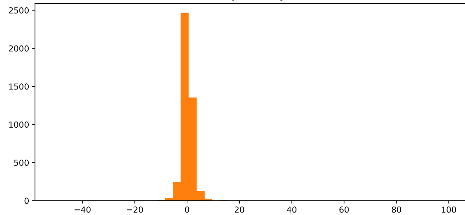
LSTM Forecast
