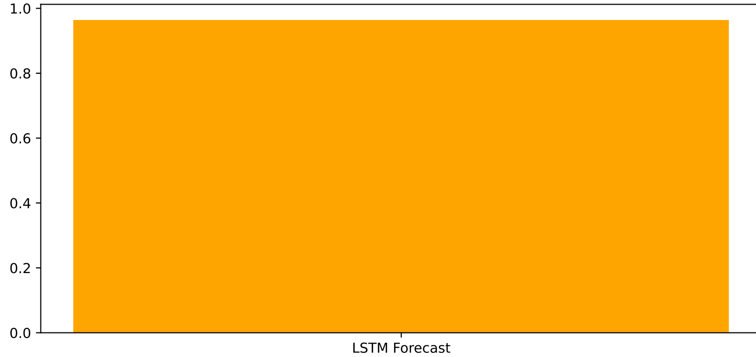
LSTM Forecast
