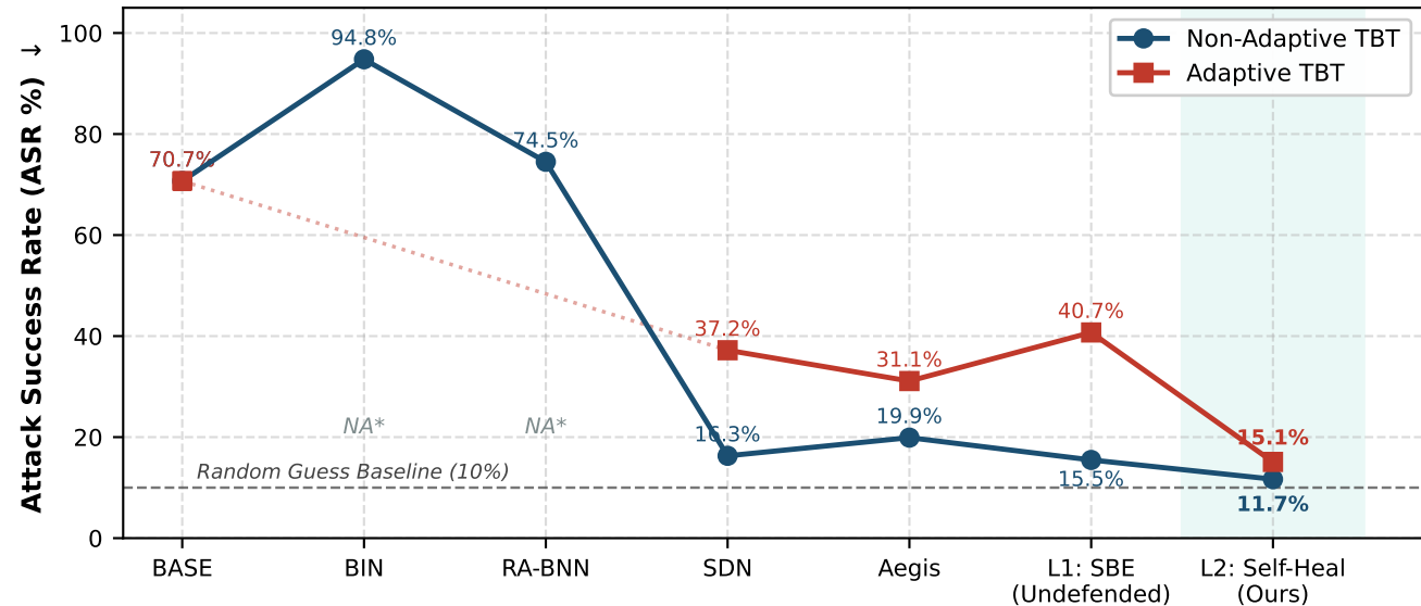
TBT Attack Success Rate (ASR) Across Defense Models on CIFAR-10 (ResNet-32)
