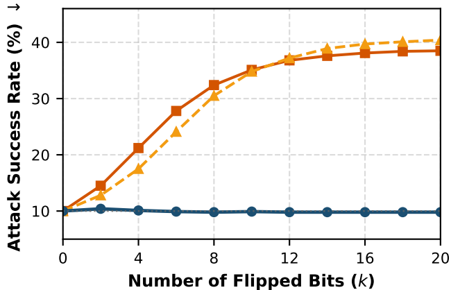
(a) ASR Progression vs. Bit-Flips
