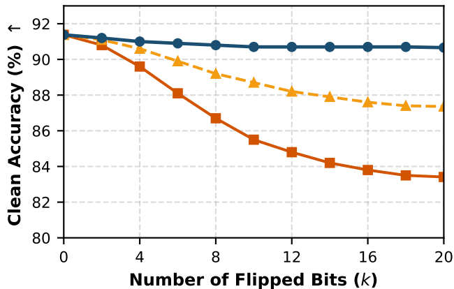
(b) Clean Accuracy Degradation vs. Bit-Flips
