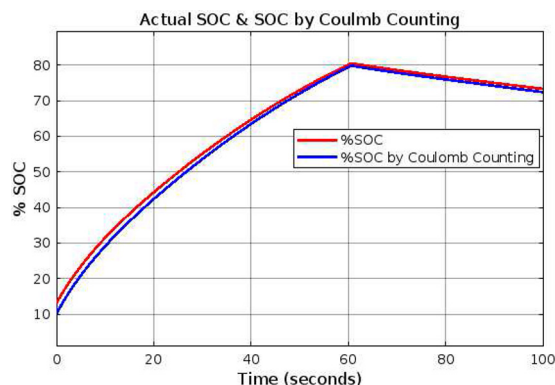
Fig. 8. Comparison of %SOC Estimation Methods
