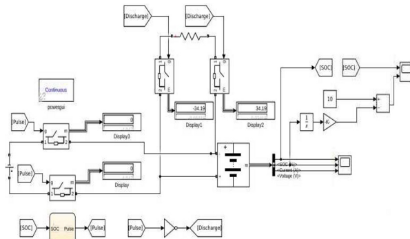
Fig. 6. Simulink Model for SOC Estimation
