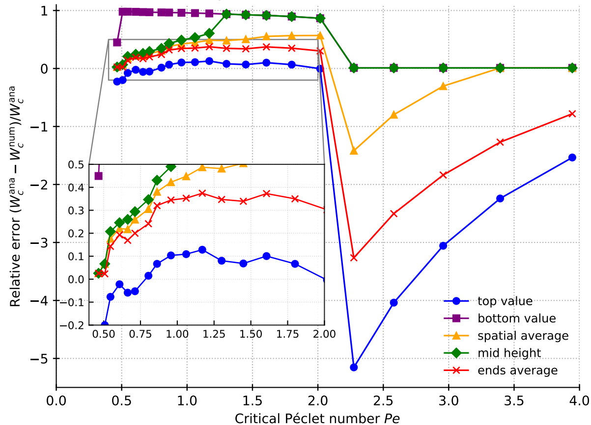
Analytical vs numerical thresholds
