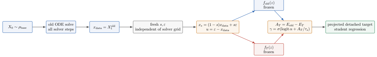
Figure 2: Full A2 pipeline. The behavior ODE supplies only the endpoint. The FM probe uses fresh randomness, and gradients belong only to the final student evaluation.
