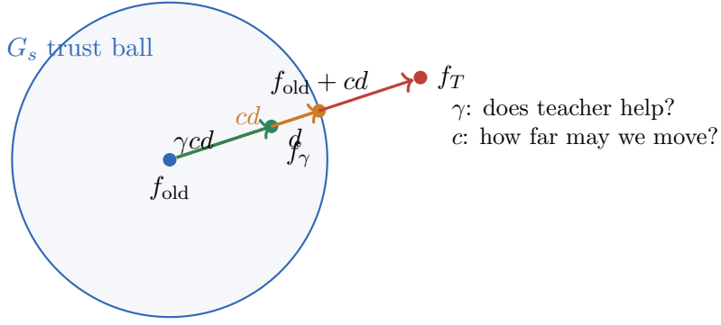
Figure 7: Trust-ball projection. The projection coefficient bounds the full teacher displacement; the gate can only shorten it further.
