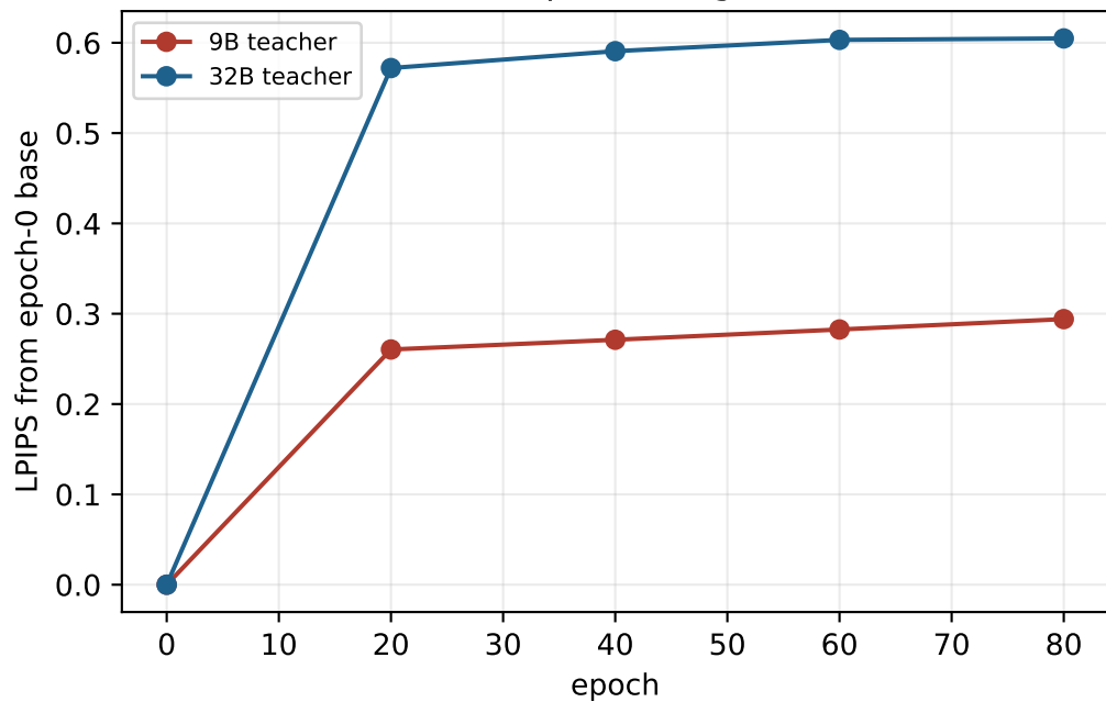
(c) Perceptual image drift
