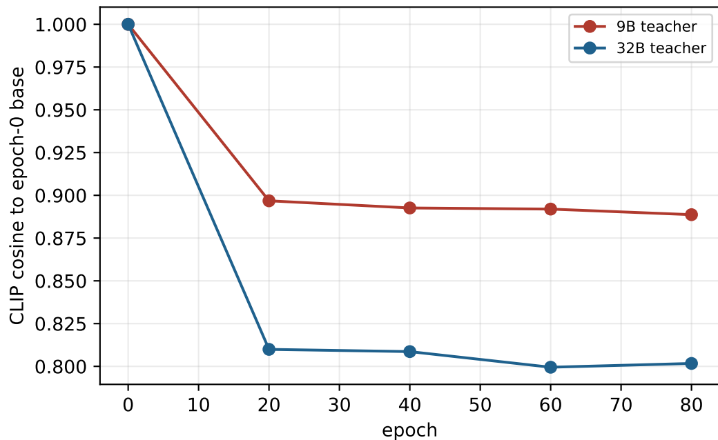
(c) Perceptual image drift
