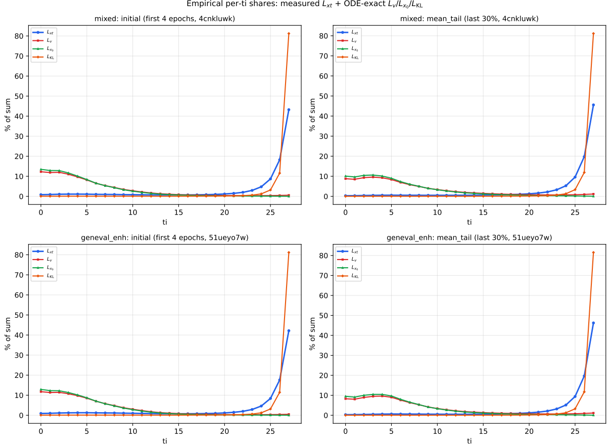
Figure 2: Empirical per-ti shares in each loss space. Top row: mixed run (4cnkluwk); bottom row: geneval_enh specialist (51ueyo7w). Left: initial window; right: mean_tail. Orange: converted L_{KL} = L_{xt}/(2\sigma_k^2) (§1.1). Late dominance is strongest in L_{KL} , absent in L_v/L_{x_0} .
