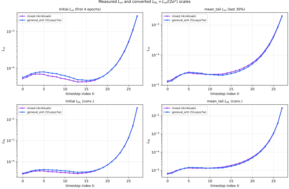
Figure 3: Top row: measured L_{xt,k} (log-y); bottom row: converted L_{KL,k} = L_{xt,k}/(2\sigma_k^2) . Both runs show the L_{xt} U-shape; L_{KL} is even more concentrated on late ti because of the 1/\sigma_k^2 factor.
