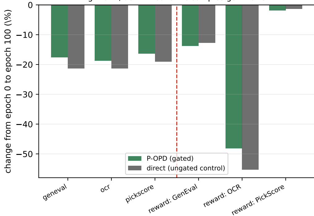
(a) left of the line, down means the objective IMPROVED; right of it, down means the samples got WORSE
