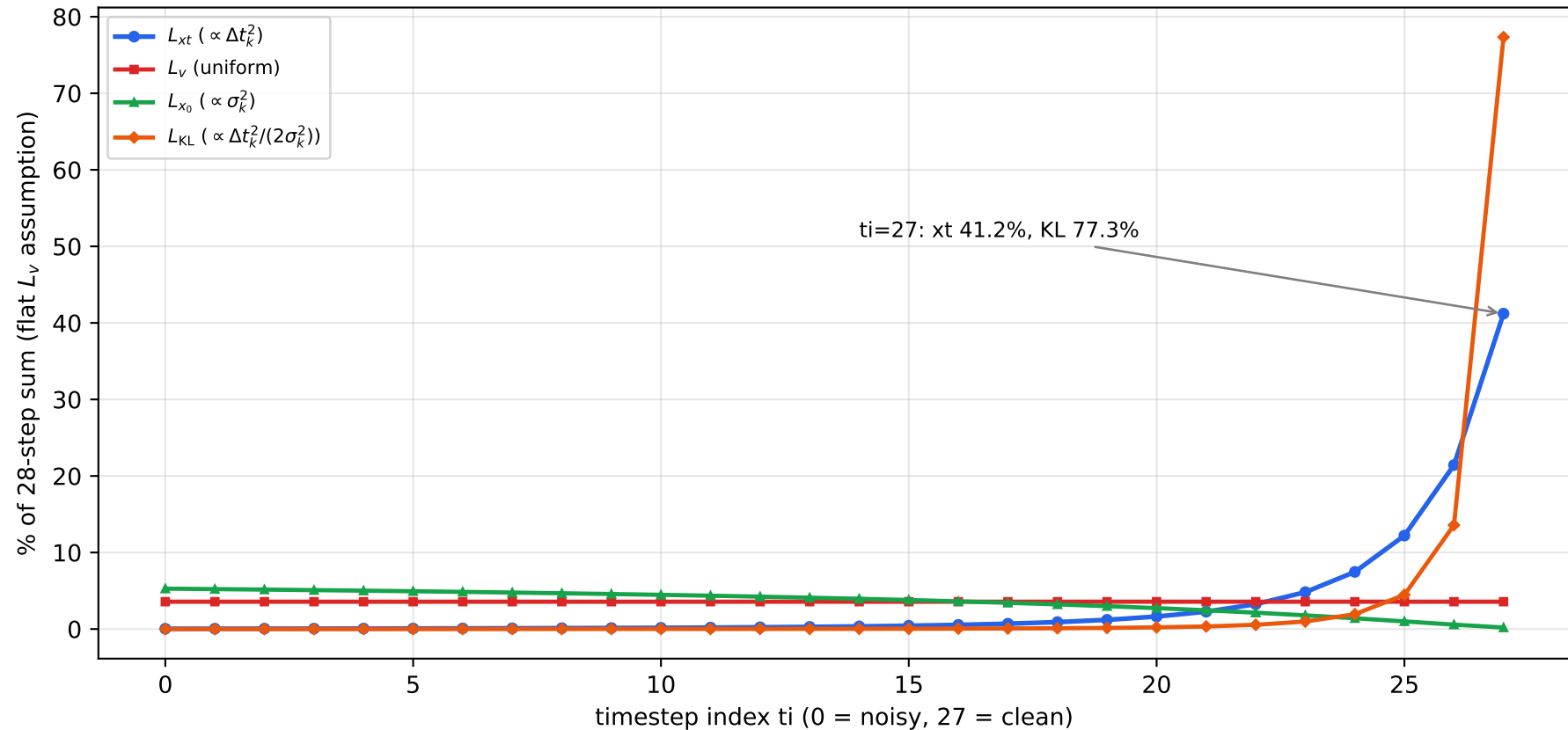
Implicit per-step shares: three MSE knobs + Gaussian transition KL
