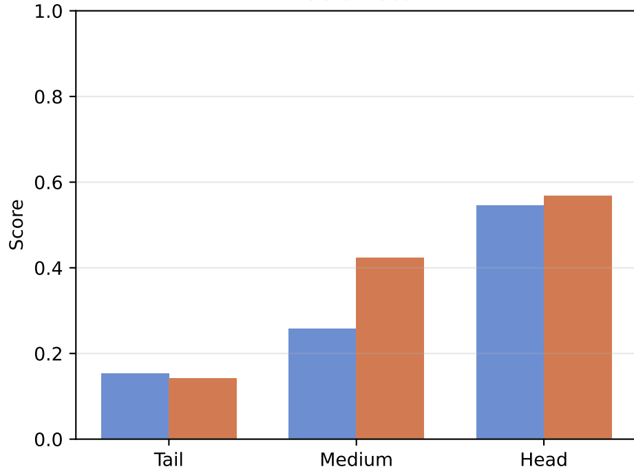
Macro Recall
